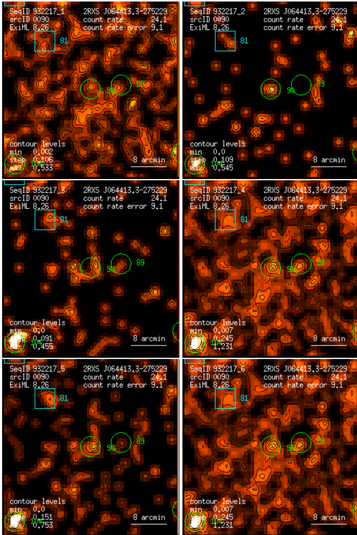
Figure 90: RASS 932217: detection 0090: band rate images, Gaussian filter: (1) PSPC channels 11 – 41, (2) 52 – 90, (3) 91 – 201, (4) 11 – 235, (5) 52 – 201, (6) 11 – 201. Broad band rates in counts/ks. Band rate contour levels in counts/ks/arcmin 2 .
