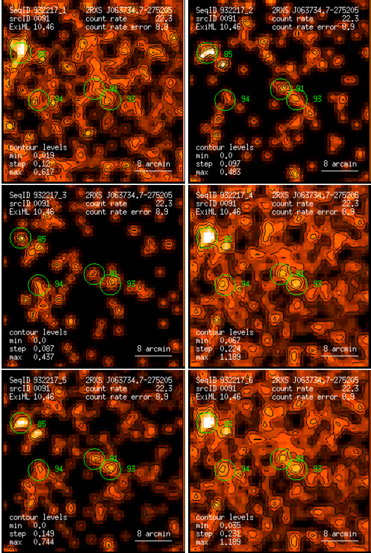
Figure 91: RASS 932217: detection 0091: band rate images, Gaussian filter: (1) PSPC channels 11 – 41, (2) 52 – 90, (3) 91 – 201, (4) 11 – 235, (5) 52 – 201, (6) 11 – 201. Broad band rates in counts/ks. Band rate contour levels in counts/ks/arcmin 2 .
