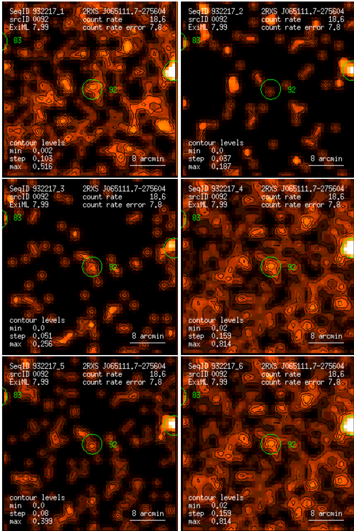
Figure 92: RASS 932217: detection 0092: band rate images, Gaussian filter: (1) PSPC channels 11 – 41, (2) 52 – 90, (3) 91 – 201, (4) 11 – 235, (5) 52 – 201, (6) 11 – 201. Broad band rates in counts/ks. Band rate contour levels in counts/ks/arcmin 2 .
