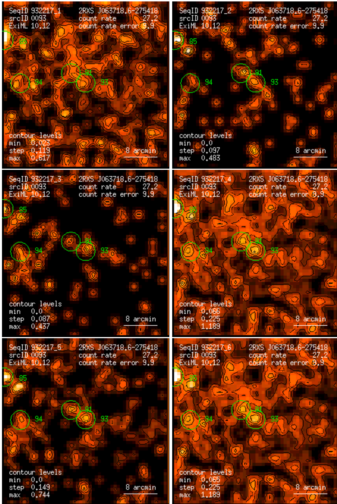
Figure 93: RASS 932217: detection 0093: band rate images, Gaussian filter: (1) PSPC channels 11 – 41, (2) 52 – 90, (3) 91 – 201, (4) 11 – 235, (5) 52 – 201, (6) 11 – 201. Broad band rates in counts/ks. Band rate contour levels in counts/ks/arcmin 2 .
