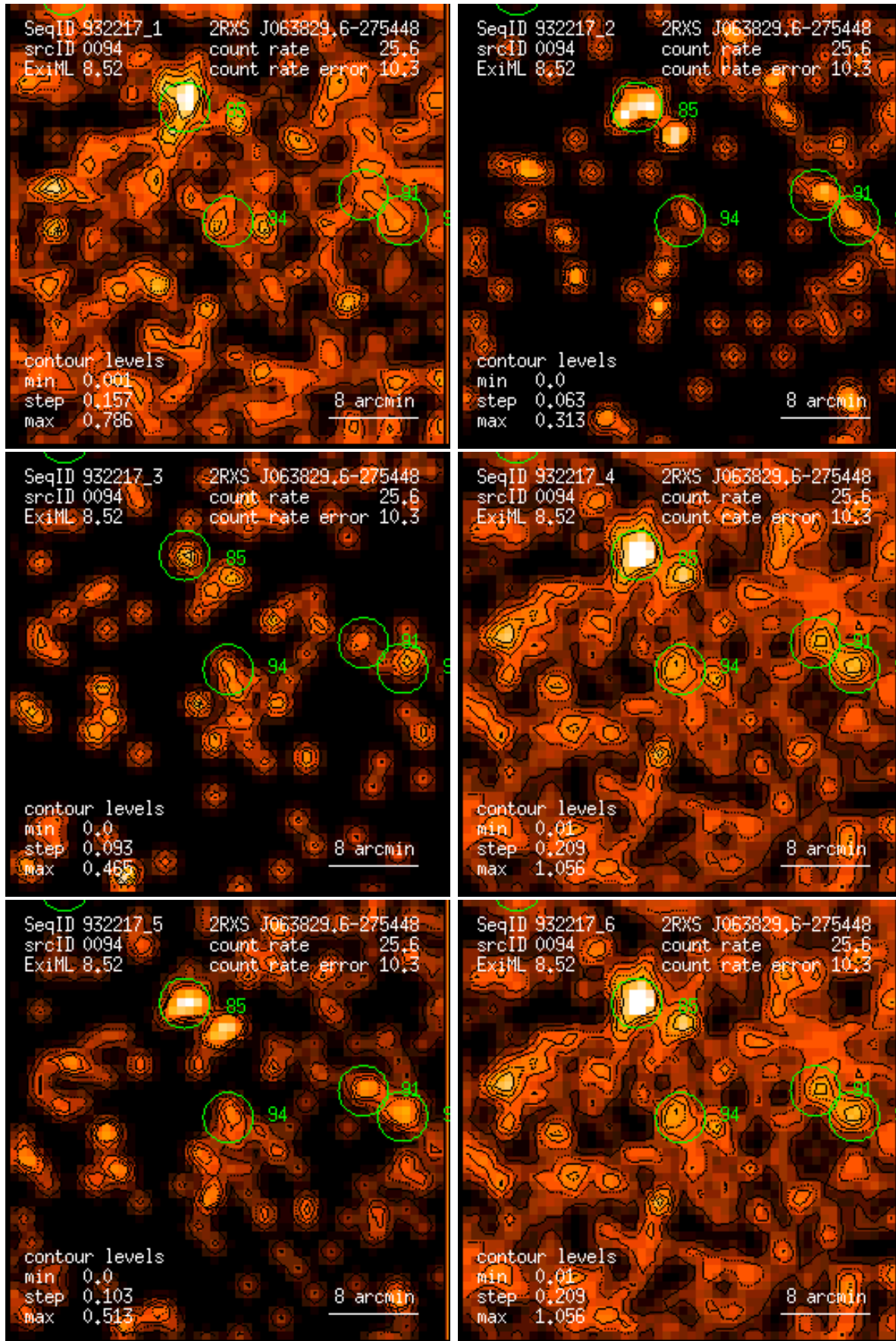
Figure 94: RASS 932217: detection 0094: band rate images, Gaussian filter: (1) PSPC channels 11 – 41, (2) 52 – 90, (3) 91 – 201, (4) 11 – 235, (5) 52 – 201, (6) 11 – 201. Broad band rates in counts/ks. Band rate contour levels in counts/ks/arcmin 2 .
