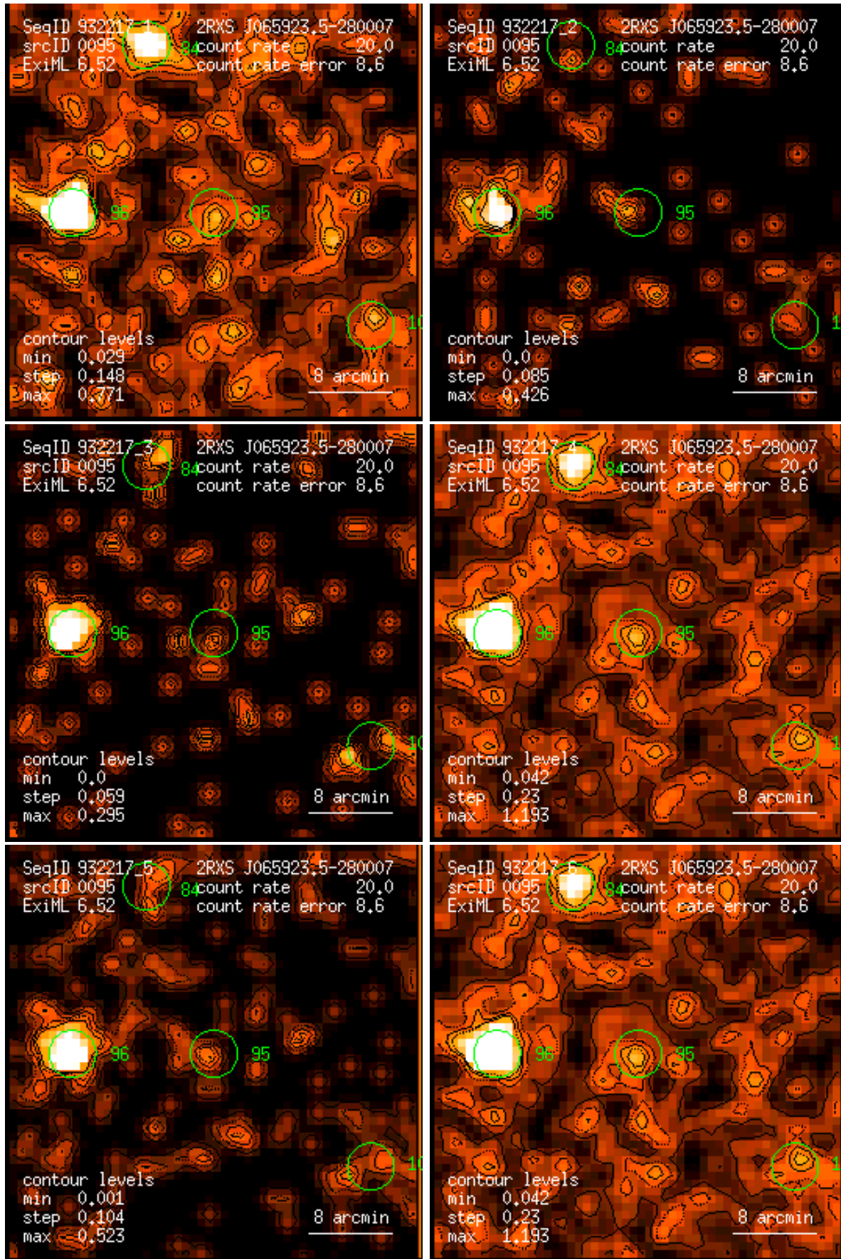
Figure 95: RASS 932217: detection 0095: band rate images, Gaussian filter: (1) PSPC channels 11 – 41, (2) 52 – 90, (3) 91 – 201, (4) 11 – 235, (5) 52 – 201, (6) 11 – 201. Broad band rates in counts/ks. Band rate contour levels in counts/ks/arcmin 2 .
