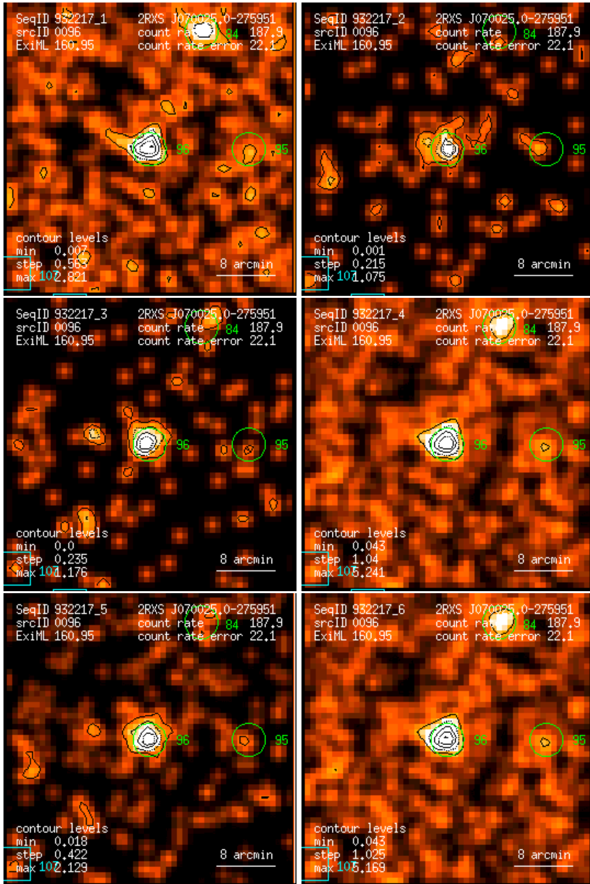
Figure 96: RASS 932217: detection 0096: band rate images, Gaussian filter: (1) PSPC channels 11 – 41, (2) 52 – 90, (3) 91 – 201, (4) 11 – 235, (5) 52 – 201, (6) 11 – 201. Broad band rates in counts/ks. Band rate contour levels in counts/ks/arcmin 2 .
