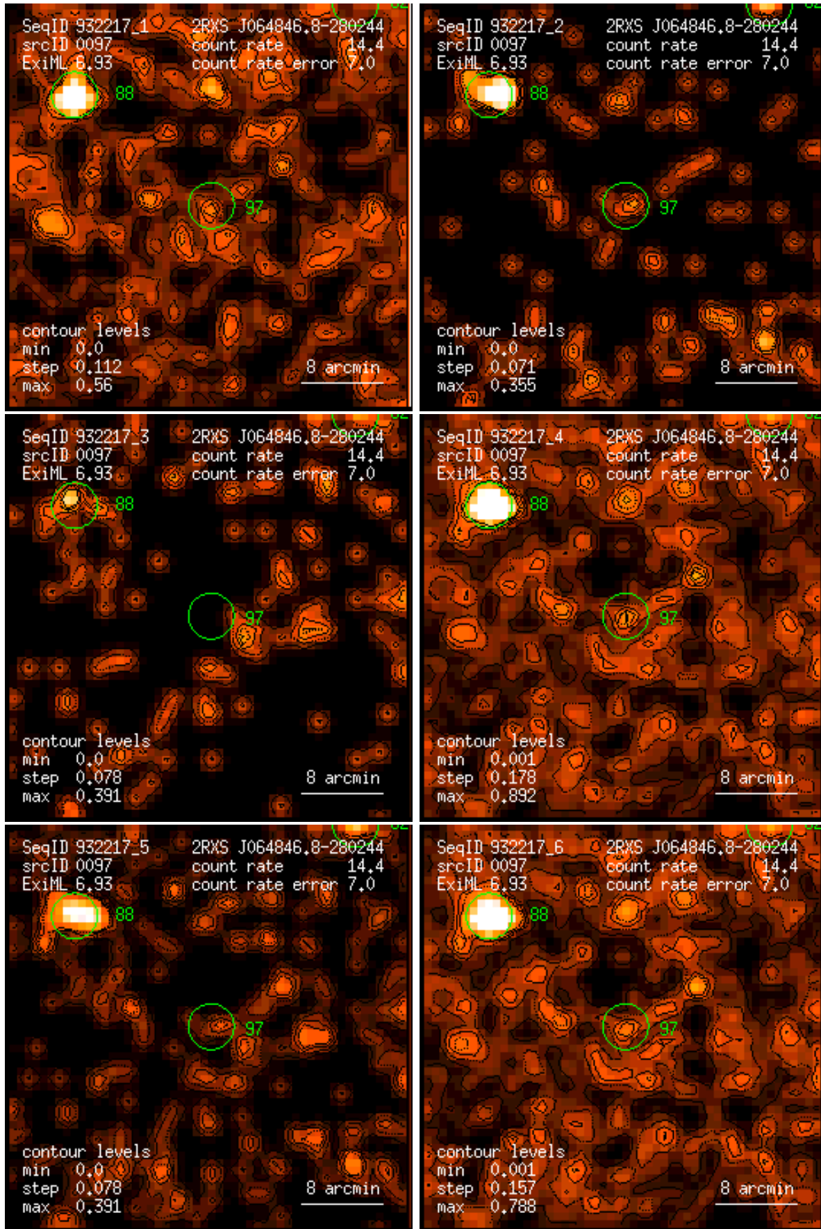
Figure 97: RASS 932217: detection 0097: band rate images, Gaussian filter: (1) PSPC channels 11 – 41, (2) 52 – 90, (3) 91 – 201, (4) 11 – 235, (5) 52 – 201, (6) 11 – 201. Broad band rates in counts/ks. Band rate contour levels in counts/ks/arcmin 2 .
