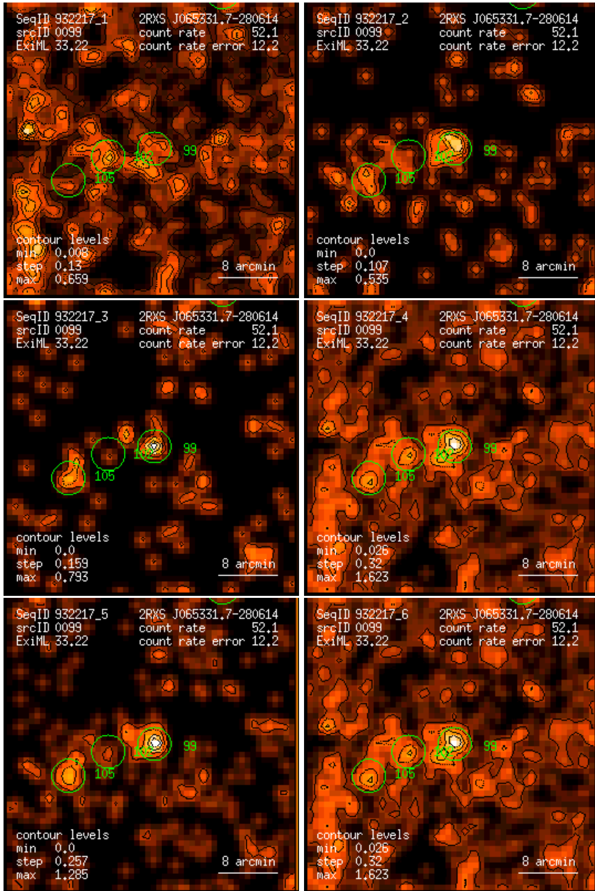
Figure 99: RASS 932217: detection 0099: band rate images, Gaussian filter: (1) PSPC channels 11 – 41, (2) 52 – 90, (3) 91 – 201, (4) 11 – 235, (5) 52 – 201, (6) 11 – 201. Broad band rates in counts/ks. Band rate contour levels in counts/ks/arcmin 2 .
