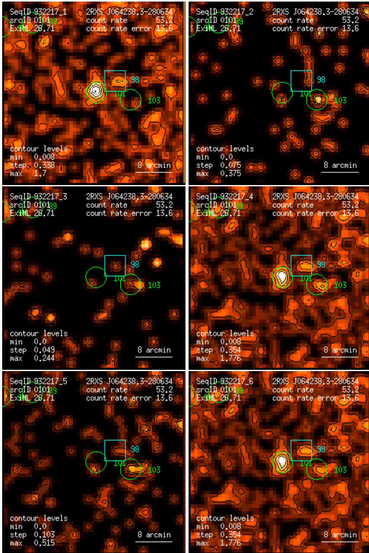
Figure 101: RASS 932217: detection 0101: band rate images, Gaussian filter: (1) PSPC channels 11 – 41, (2) 52 – 90, (3) 91 – 201, (4) 11 – 235, (5) 52 – 201, (6) 11 – 201. Broad band rates in counts/ks. Band rate contour levels in counts/ks/arcmin 2 .
