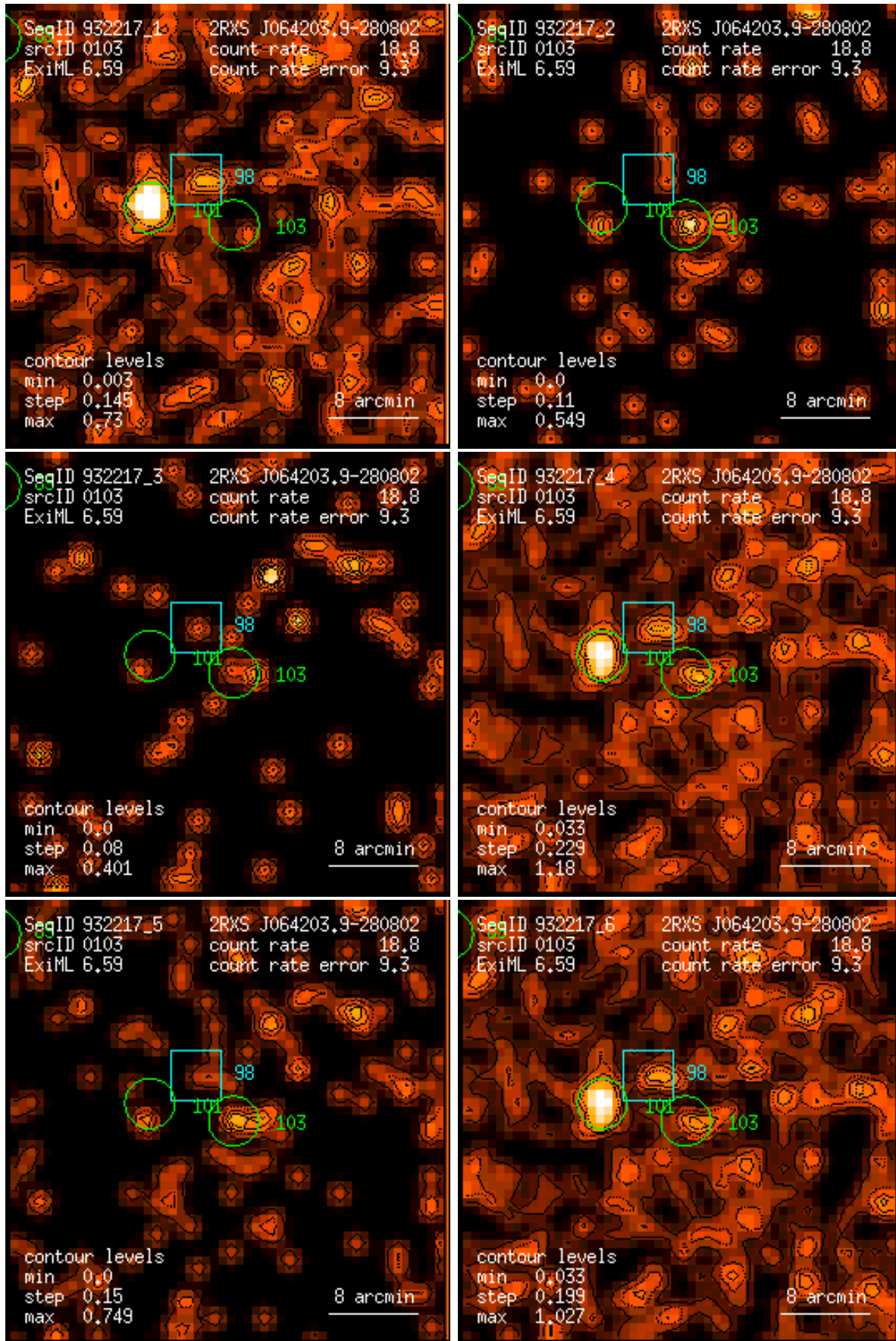
Figure 103: RASS 932217: detection 0103: band rate images, Gaussian filter: (1) PSPC channels 11 – 41, (2) 52 – 90, (3) 91 – 201, (4) 11 – 235, (5) 52 – 201, (6) 11 – 201. Broad band rates in counts/ks. Band rate contour levels in counts/ks/arcmin 2 .
