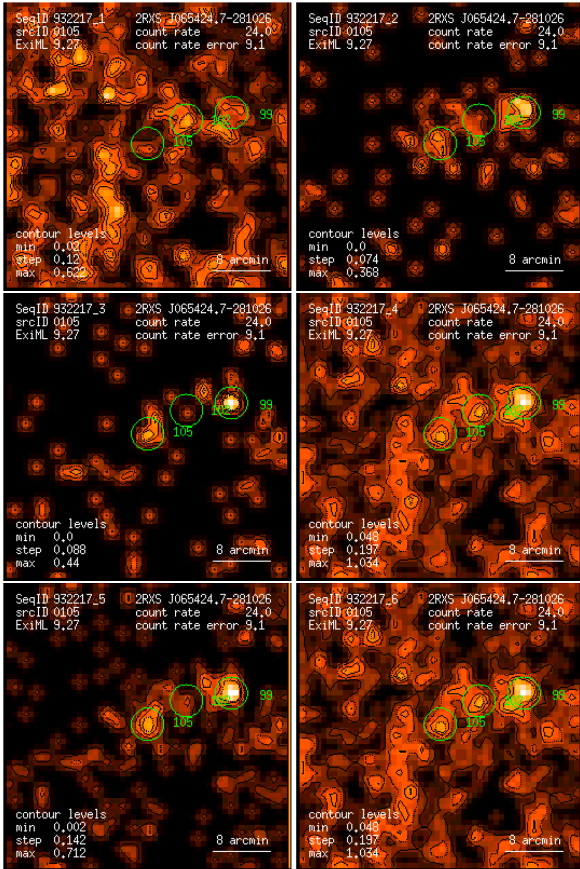
Figure 105: RASS 932217: detection 0105: band rate images, Gaussian filter: (1) PSPC channels 11 – 41, (2) 52 – 90, (3) 91 – 201, (4) 11 – 235, (5) 52 – 201, (6) 11 – 201. Broad band rates in counts/ks. Band rate contour levels in counts/ks/arcmin 2 .
