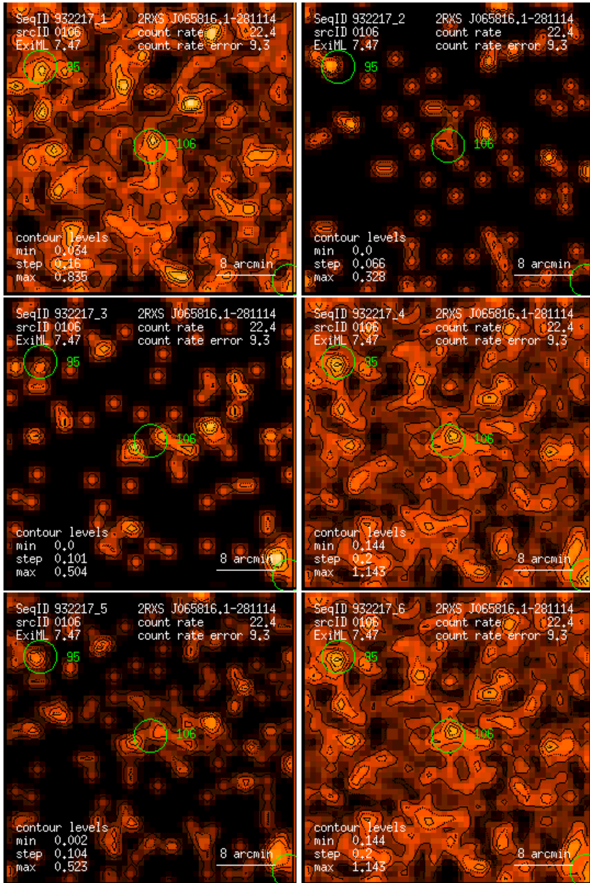
Figure 106: RASS 932217: detection 0106: band rate images, Gaussian filter: (1) PSPC channels 11 – 41, (2) 52 – 90, (3) 91 – 201, (4) 11 – 235, (5) 52 – 201, (6) 11 – 201. Broad band rates in counts/ks. Band rate contour levels in counts/ks/arcmin 2 .
