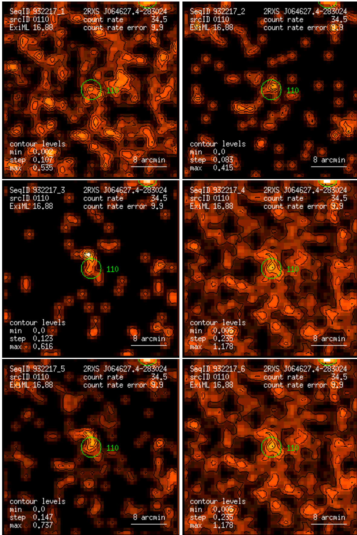
Figure 110: RASS 932217: detection 0110: band rate images, Gaussian filter: (1) PSPC channels 11 – 41, (2) 52 – 90, (3) 91 – 201, (4) 11 – 235, (5) 52 – 201, (6) 11 – 201. Broad band rates in counts/ks. Band rate contour levels in counts/ks/arcmin 2 .
