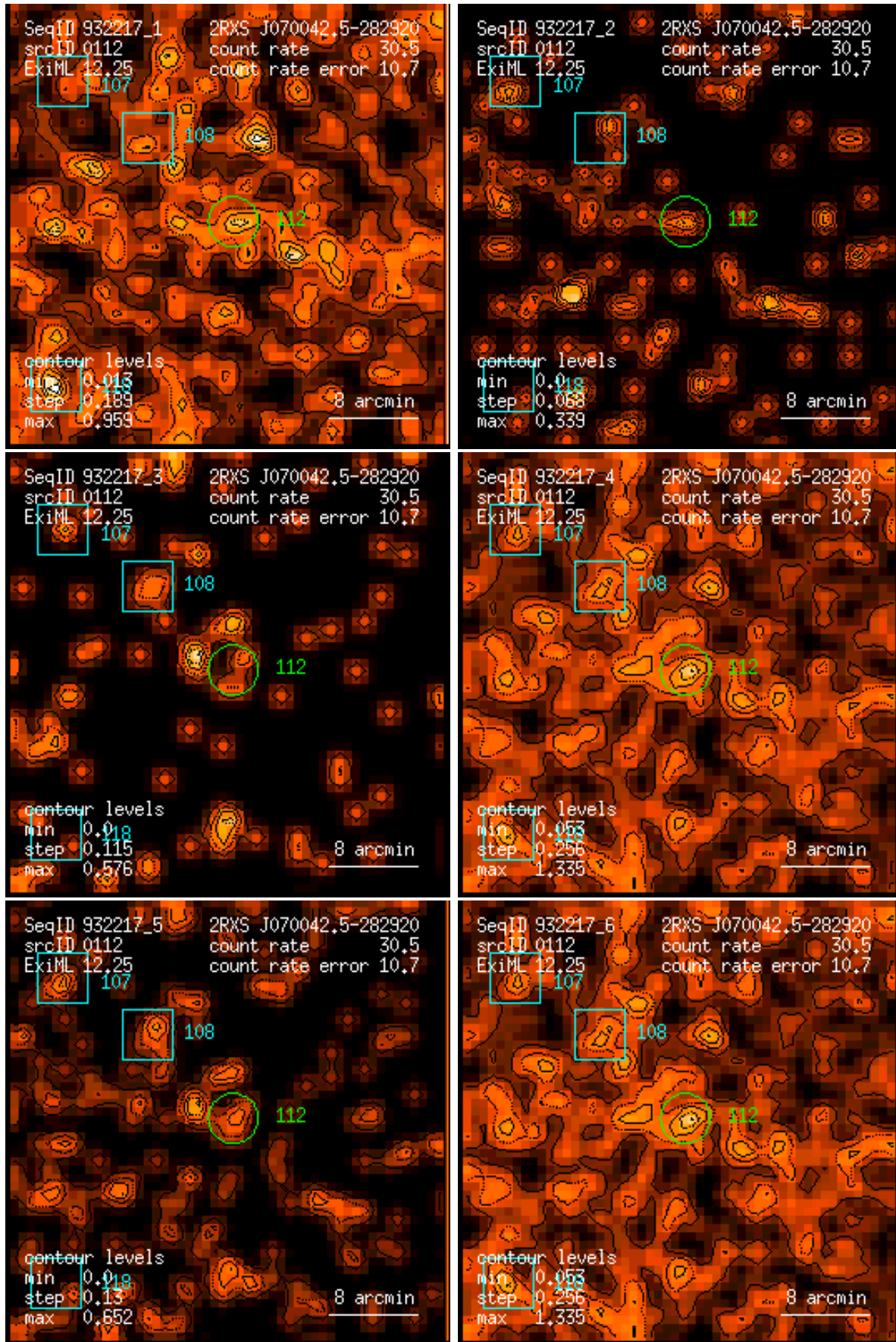
Figure 112: RASS 932217: detection 0112: band rate images, Gaussian filter: (1) PSPC channels 11 – 41, (2) 52 – 90, (3) 91 – 201, (4) 11 – 235, (5) 52 – 201, (6) 11 – 201. Broad band rates in counts/ks. Band rate contour levels in counts/ks/arcmin 2 .
