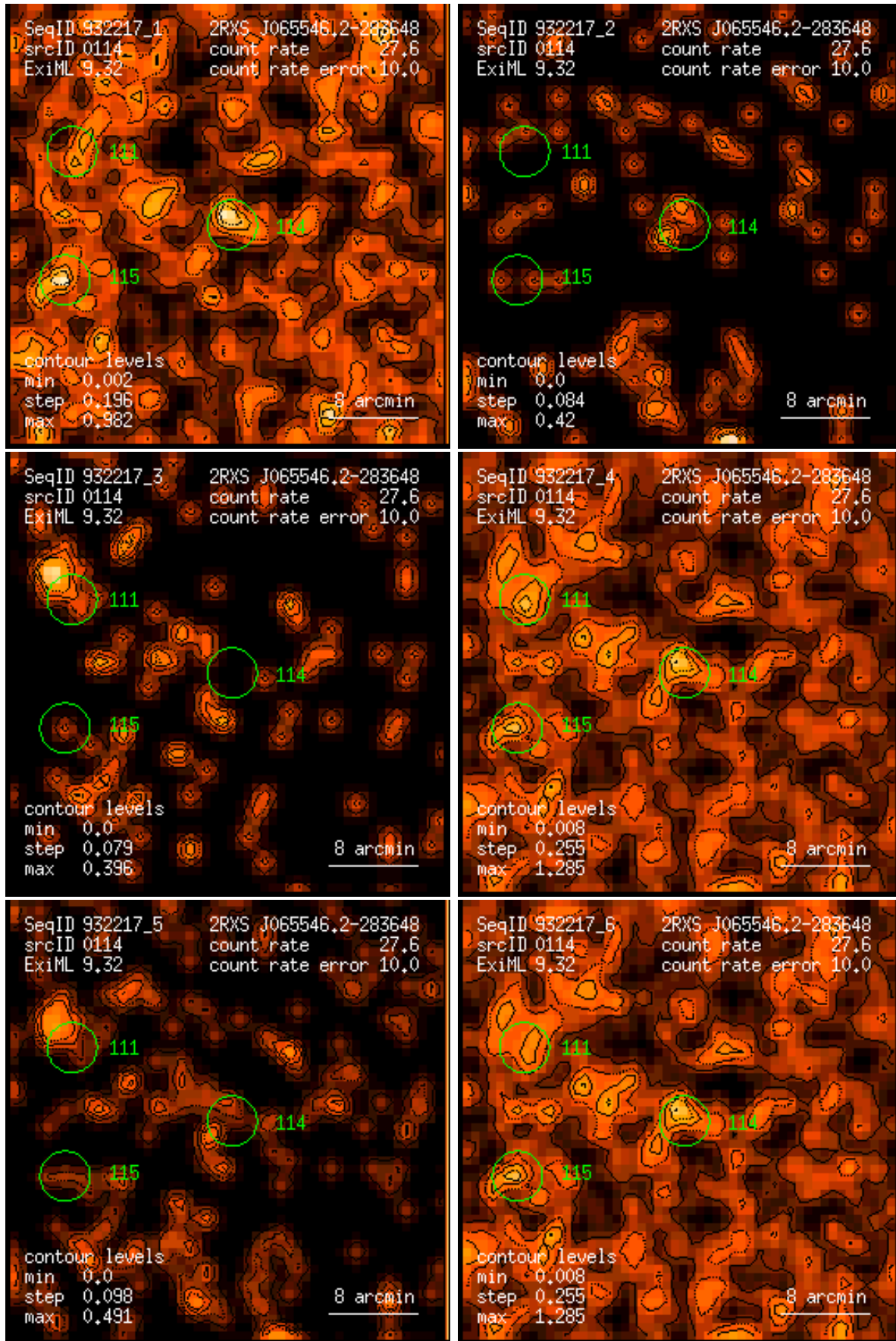
Figure 114: RASS 932217: detection 0114: band rate images, Gaussian filter: (1) PSPC channels 11 – 41, (2) 52 – 90, (3) 91 – 201, (4) 11 – 235, (5) 52 – 201, (6) 11 – 201. Broad band rates in counts/ks. Band rate contour levels in counts/ks/arcmin 2 .
