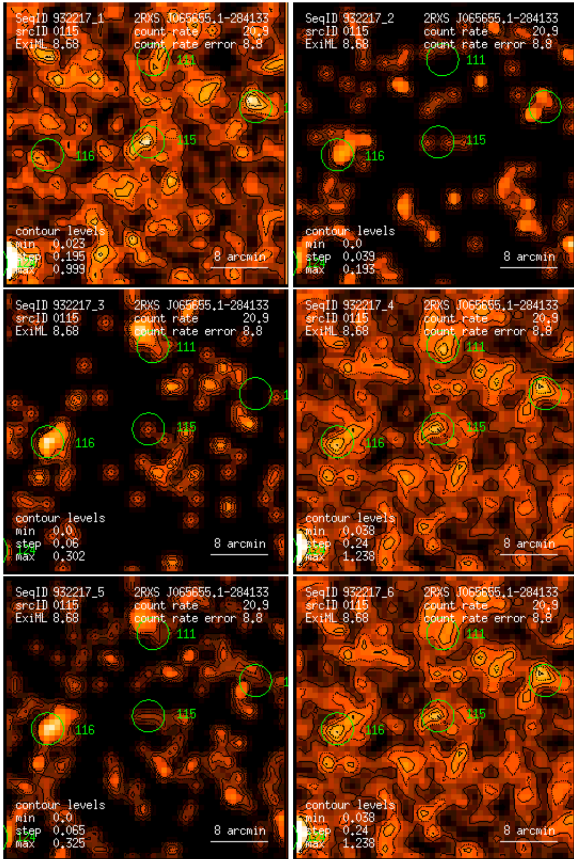
Figure 115: RASS 932217: detection 0115: band rate images, Gaussian filter: (1) PSPC channels 11 – 41, (2) 52 – 90, (3) 91 – 201, (4) 11 – 235, (5) 52 – 201, (6) 11 – 201. Broad band rates in counts/ks. Band rate contour levels in counts/ks/arcmin 2 .
