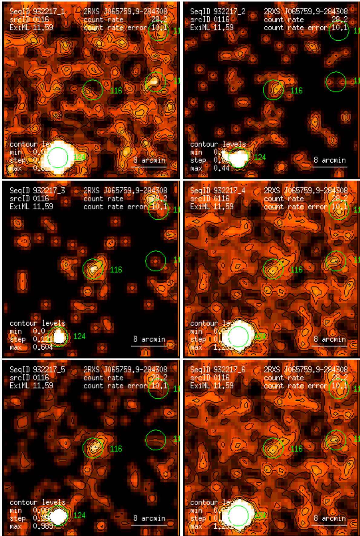
Figure 116: RASS 932217: detection 0116: band rate images, Gaussian filter: (1) PSPC channels 11 – 41, (2) 52 – 90, (3) 91 – 201, (4) 11 – 235, (5) 52 – 201, (6) 11 – 201. Broad band rates in counts/ks. Band rate contour levels in counts/ks/arcmin 2 .
