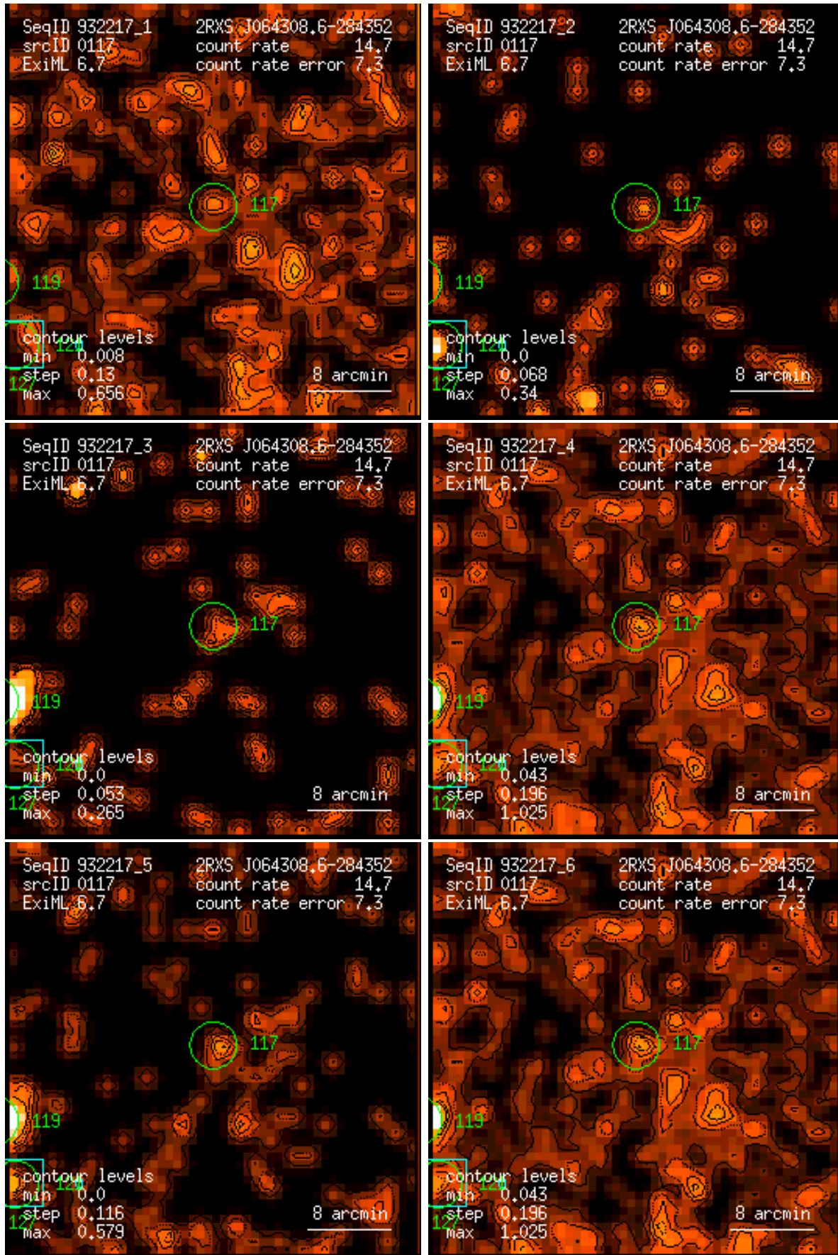
Figure 117: RASS 932217: detection 0117: band rate images, Gaussian filter: (1) PSPC channels 11 – 41, (2) 52 – 90, (3) 91 – 201, (4) 11 – 235, (5) 52 – 201, (6) 11 – 201. Broad band rates in counts/ks. Band rate contour levels in counts/ks/arcmin 2 .
