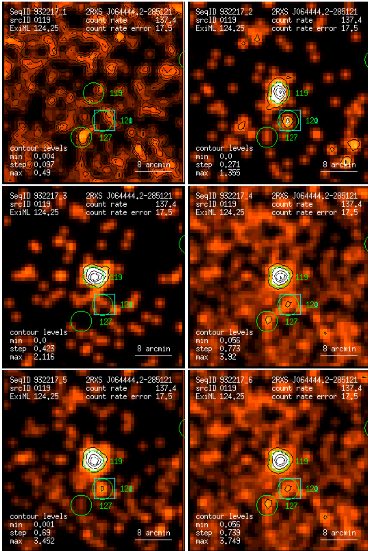
Figure 119: RASS 932217: detection 0119: band rate images, Gaussian filter: (1) PSPC channels 11 – 41, (2) 52 – 90, (3) 91 – 201, (4) 11 – 235, (5) 52 – 201, (6) 11 – 201. Broad band rates in counts/ks. Band rate contour levels in counts/ks/arcmin 2 .
