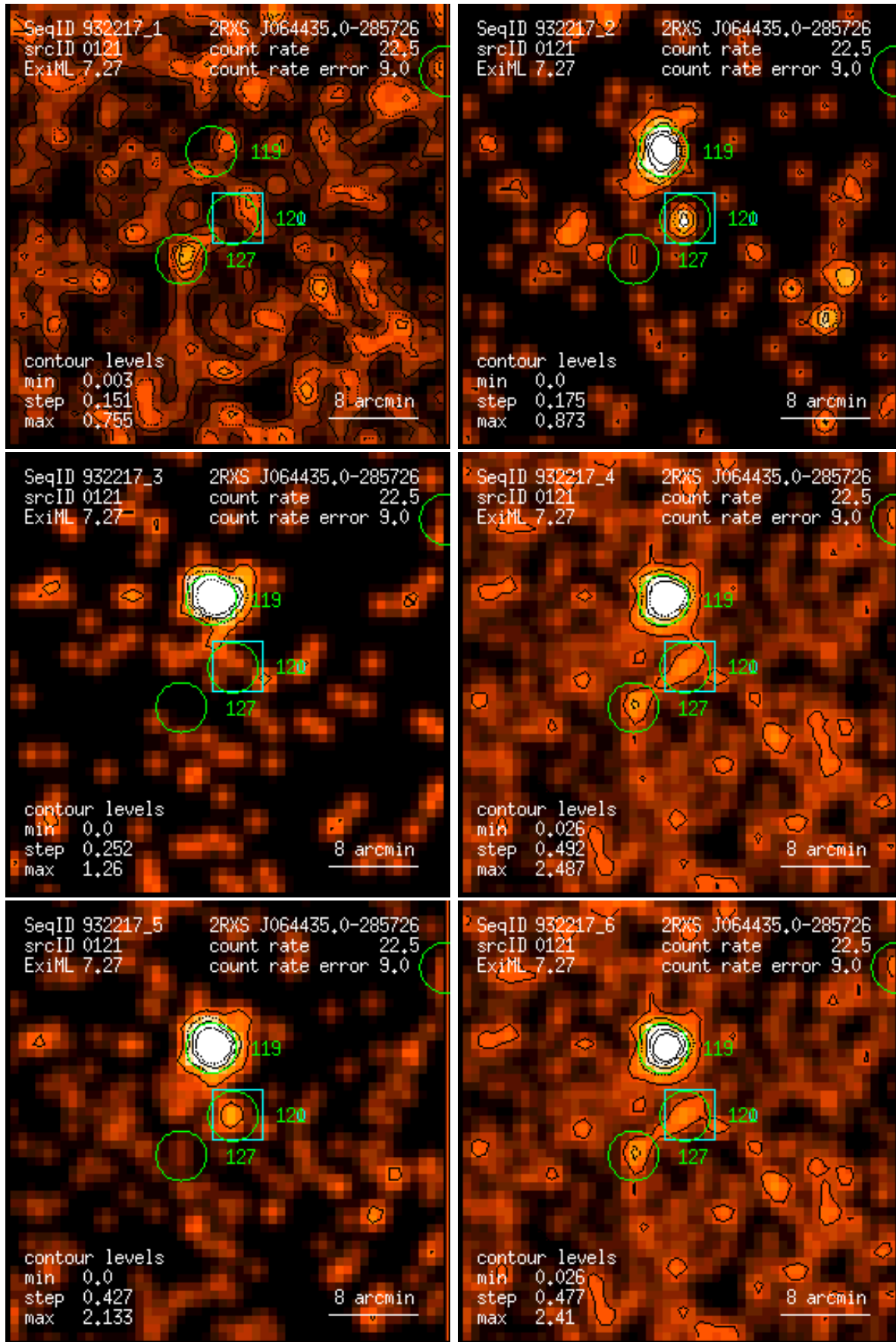
Figure 121: RASS 932217: detection 0121: band rate images, Gaussian filter: (1) PSPC channels 11 – 41, (2) 52 – 90, (3) 91 – 201, (4) 11 – 235, (5) 52 – 201, (6) 11 – 201. Broad band rates in counts/ks. Band rate contour levels in counts/ks/arcmin 2 .
