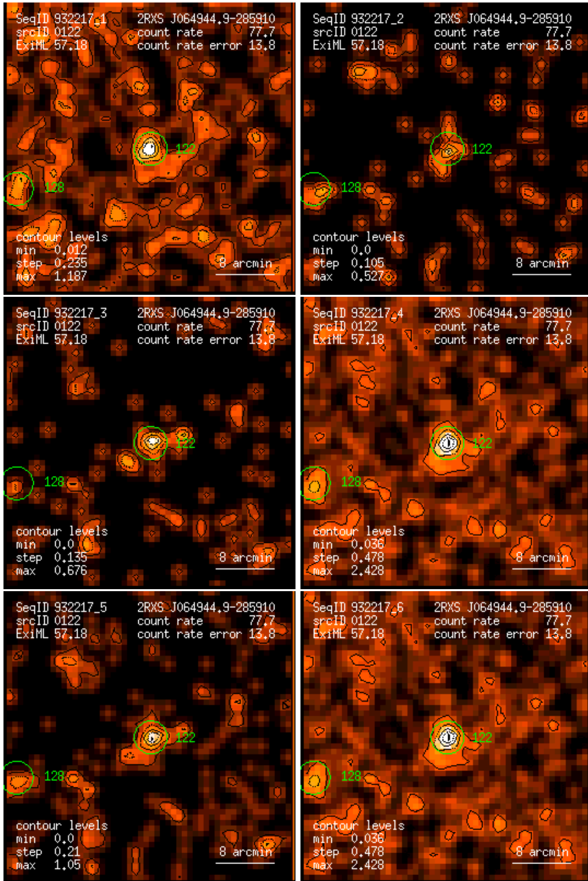
Figure 122: RASS 932217: detection 0122: band rate images, Gaussian filter: (1) PSPC channels 11 – 41, (2) 52 – 90, (3) 91 – 201, (4) 11 – 235, (5) 52 – 201, (6) 11 – 201. Broad band rates in counts/ks. Band rate contour levels in counts/ks/arcmin 2 .
