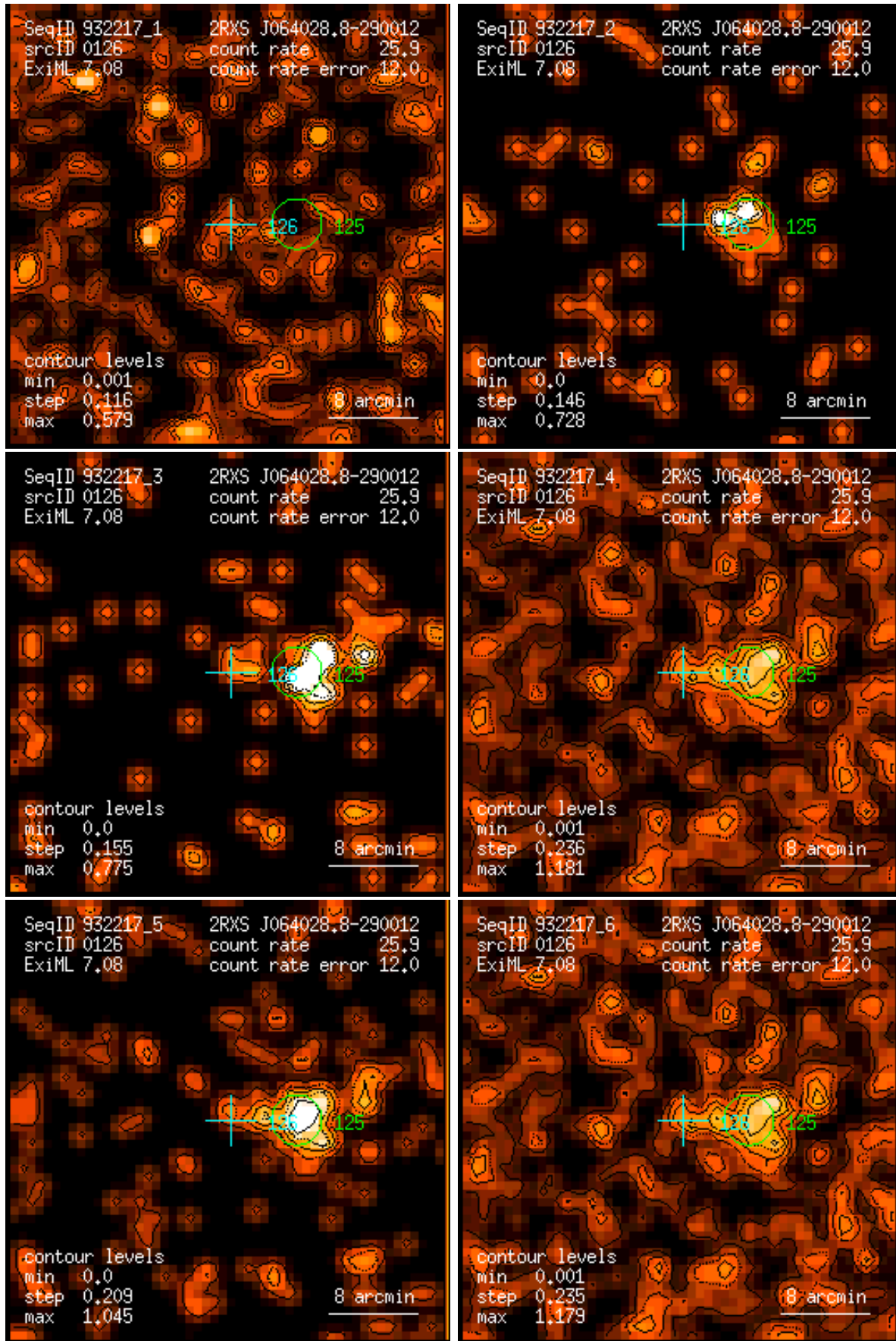
Figure 126: RASS 932217: detection 0126: band rate images, Gaussian filter: (1) PSPC channels 11 – 41, (2) 52 – 90, (3) 91 – 201, (4) 11 – 235, (5) 52 – 201, (6) 11 – 201. Broad band rates in counts/ks. Band rate contour levels in counts/ks/arcmin 2 .
