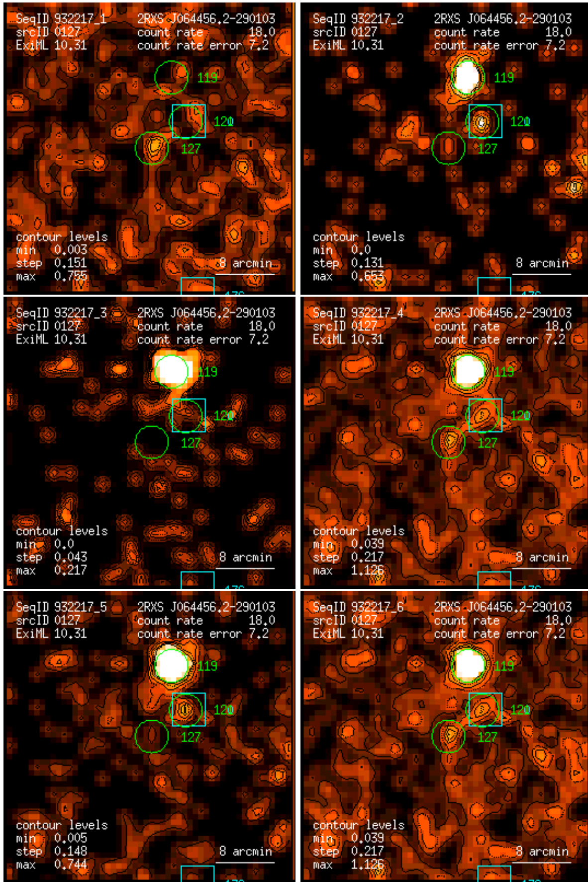
Figure 127: RASS 932217: detection 0127: band rate images, Gaussian filter: (1) PSPC channels 11 – 41, (2) 52 – 90, (3) 91 – 201, (4) 11 – 235, (5) 52 – 201, (6) 11 – 201. Broad band rates in counts/ks. Band rate contour levels in counts/ks/arcmin 2 .
