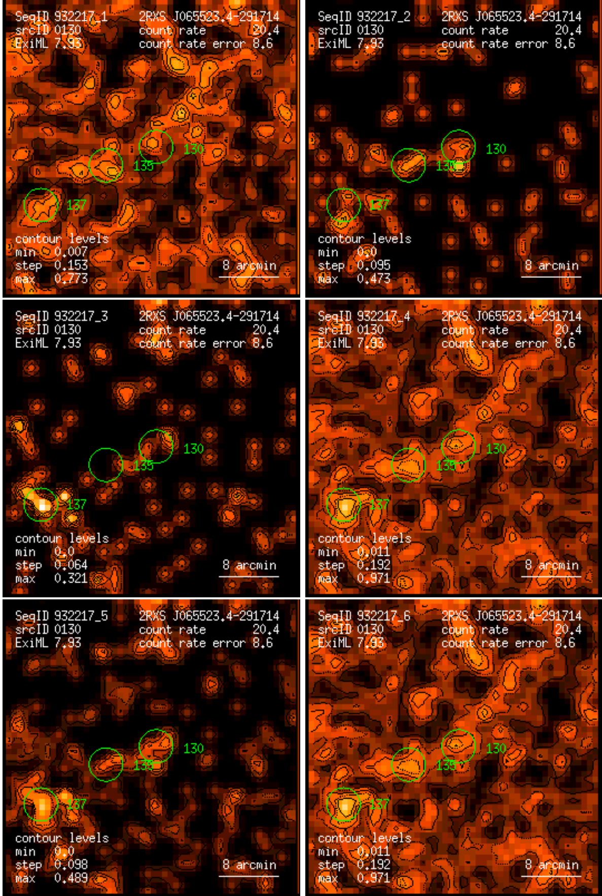
Figure 130: RASS 932217: detection 0130: band rate images, Gaussian filter: (1) PSPC channels 11 – 41, (2) 52 – 90, (3) 91 – 201, (4) 11 – 235, (5) 52 – 201, (6) 11 – 201. Broad band rates in counts/ks. Band rate contour levels in counts/ks/arcmin 2 .
