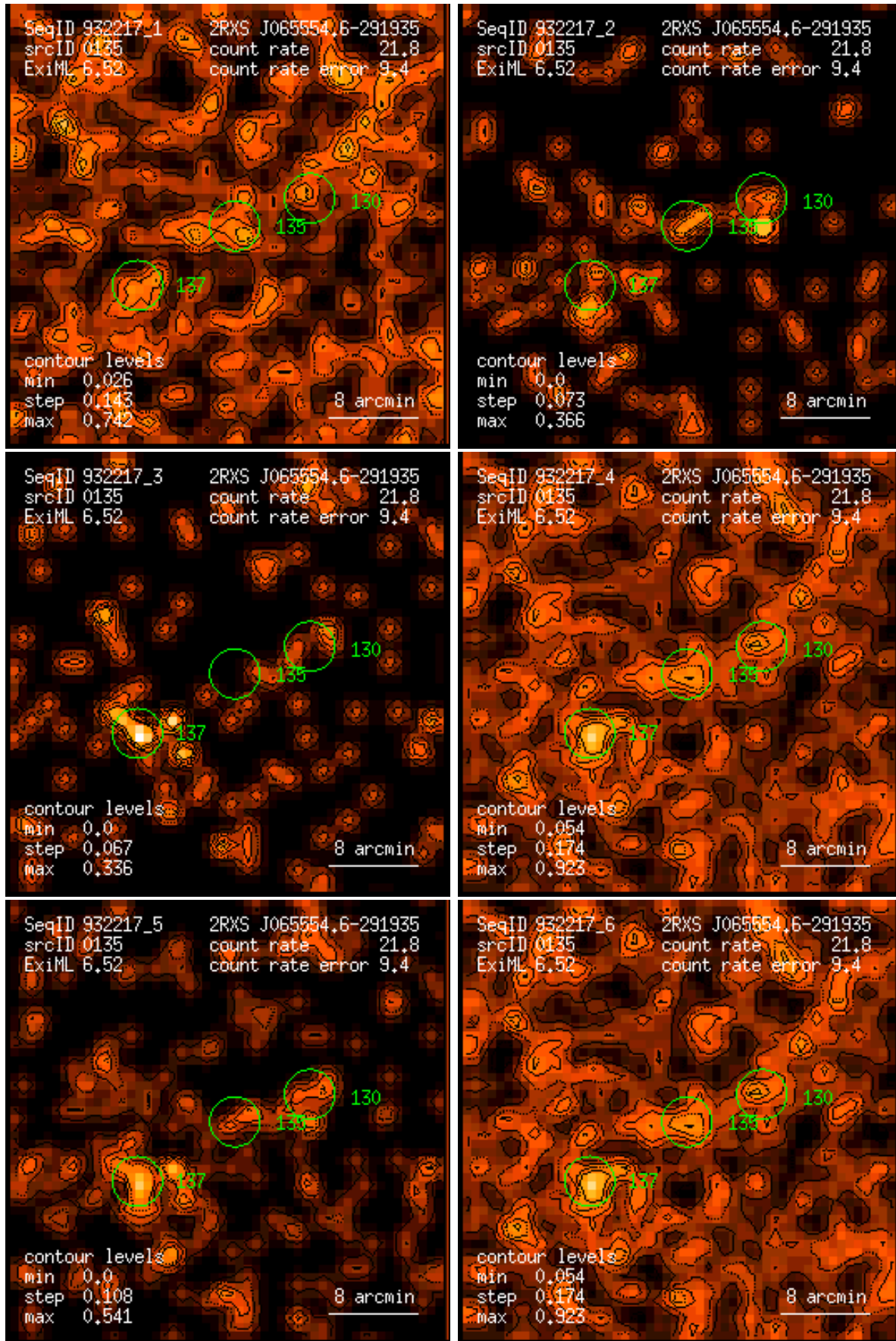
Figure 135: RASS 932217: detection 0135: band rate images, Gaussian filter: (1) PSPC channels 11 – 41, (2) 52 – 90, (3) 91 – 201, (4) 11 – 235, (5) 52 – 201, (6) 11 – 201. Broad band rates in counts/ks. Band rate contour levels in counts/ks/arcmin 2 .
