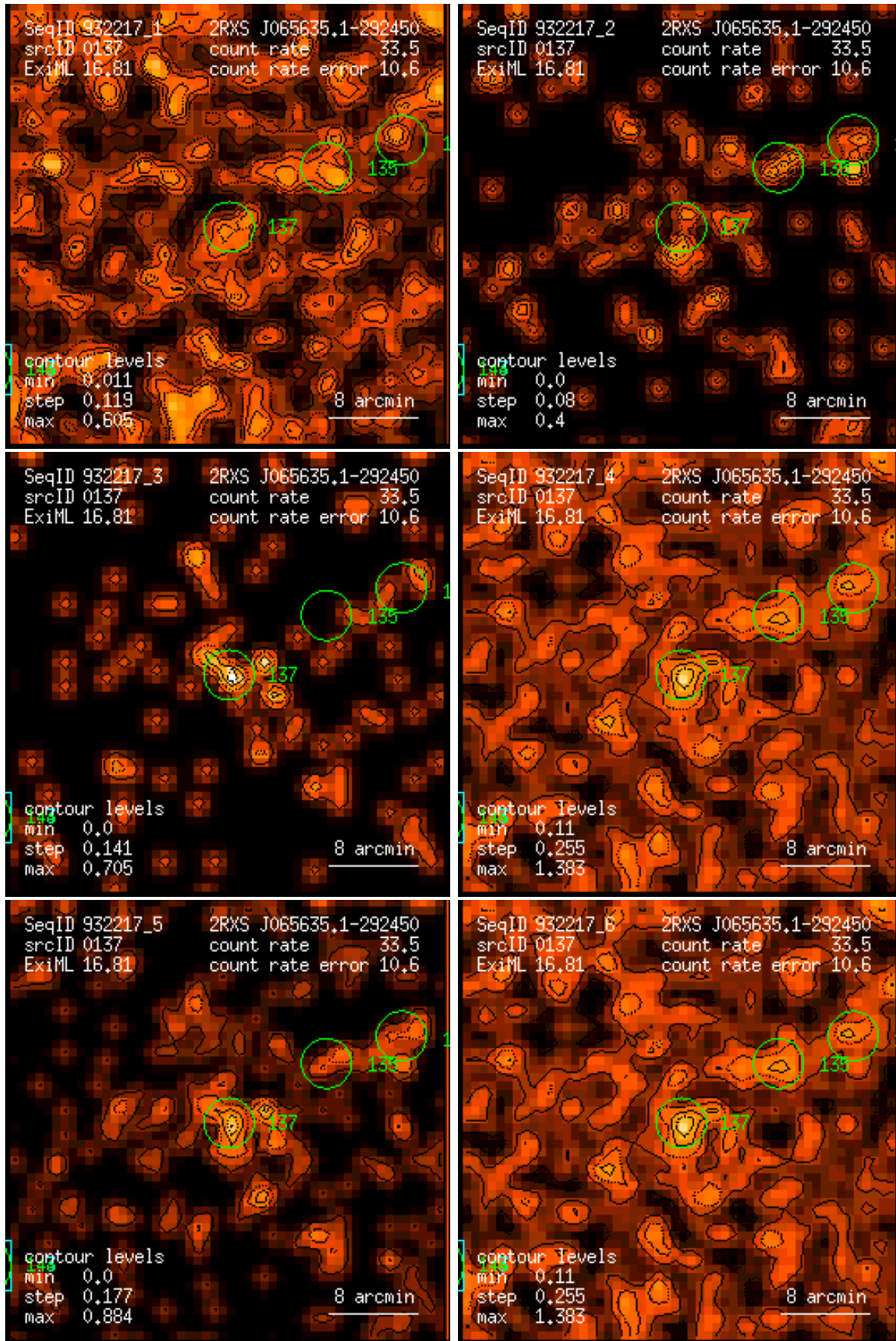
Figure 137: RASS 932217: detection 0137: band rate images, Gaussian filter: (1) PSPC channels 11 – 41, (2) 52 – 90, (3) 91 – 201, (4) 11 – 235, (5) 52 – 201, (6) 11 – 201. Broad band rates in counts/ks. Band rate contour levels in counts/ks/arcmin 2 .
