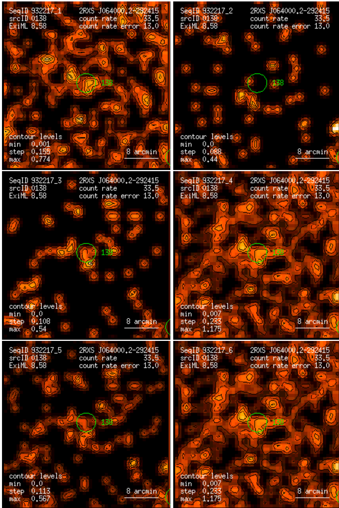
Figure 138: RASS 932217: detection 0138: band rate images, Gaussian filter: (1) PSPC channels 11 – 41, (2) 52 – 90, (3) 91 – 201, (4) 11 – 235, (5) 52 – 201, (6) 11 – 201. Broad band rates in counts/ks. Band rate contour levels in counts/ks/arcmin 2 .
