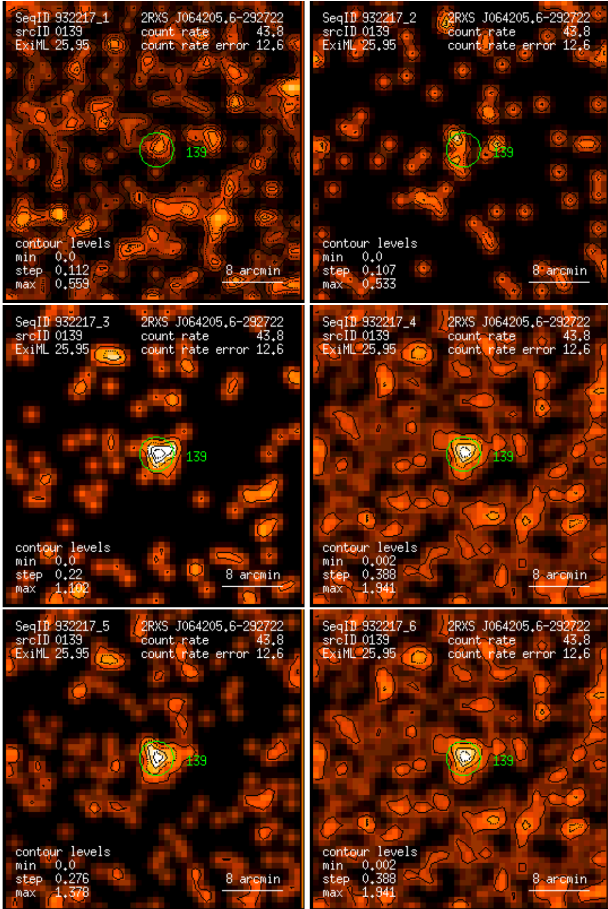
Figure 139: RASS 932217: detection 0139: band rate images, Gaussian filter: (1) PSPC channels 11 – 41, (2) 52 – 90, (3) 91 – 201, (4) 11 – 235, (5) 52 – 201, (6) 11 – 201. Broad band rates in counts/ks. Band rate contour levels in counts/ks/arcmin 2 .
