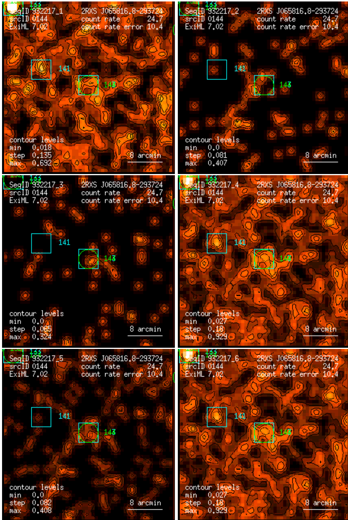
Figure 144: RASS 932217: detection 0144: band rate images, Gaussian filter: (1) PSPC channels 11 – 41, (2) 52 – 90, (3) 91 – 201, (4) 11 – 235, (5) 52 – 201, (6) 11 – 201. Broad band rates in counts/ks. Band rate contour levels in counts/ks/arcmin 2 .
