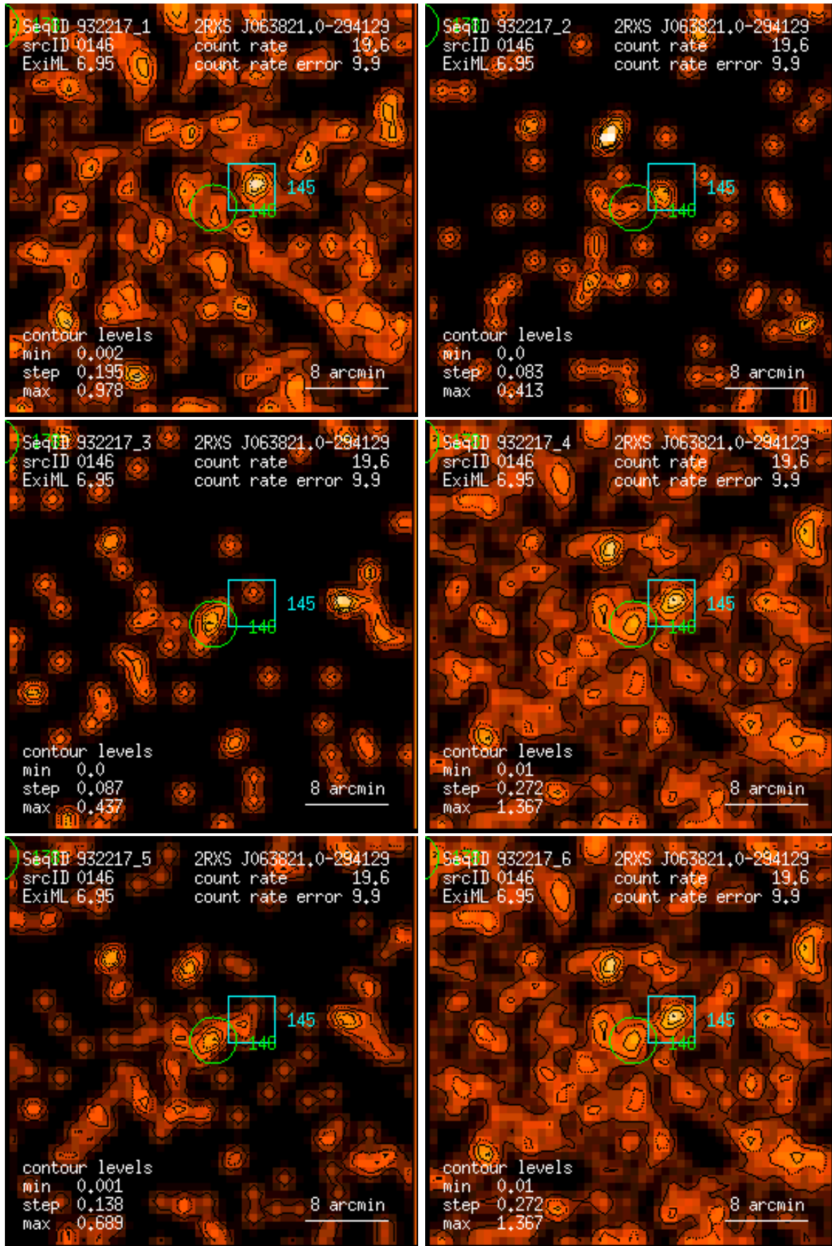
Figure 146: RASS 932217: detection 0146: band rate images, Gaussian filter: (1) PSPC channels 11 – 41, (2) 52 – 90, (3) 91 – 201, (4) 11 – 235, (5) 52 – 201, (6) 11 – 201. Broad band rates in counts/ks. Band rate contour levels in counts/ks/arcmin 2 .
