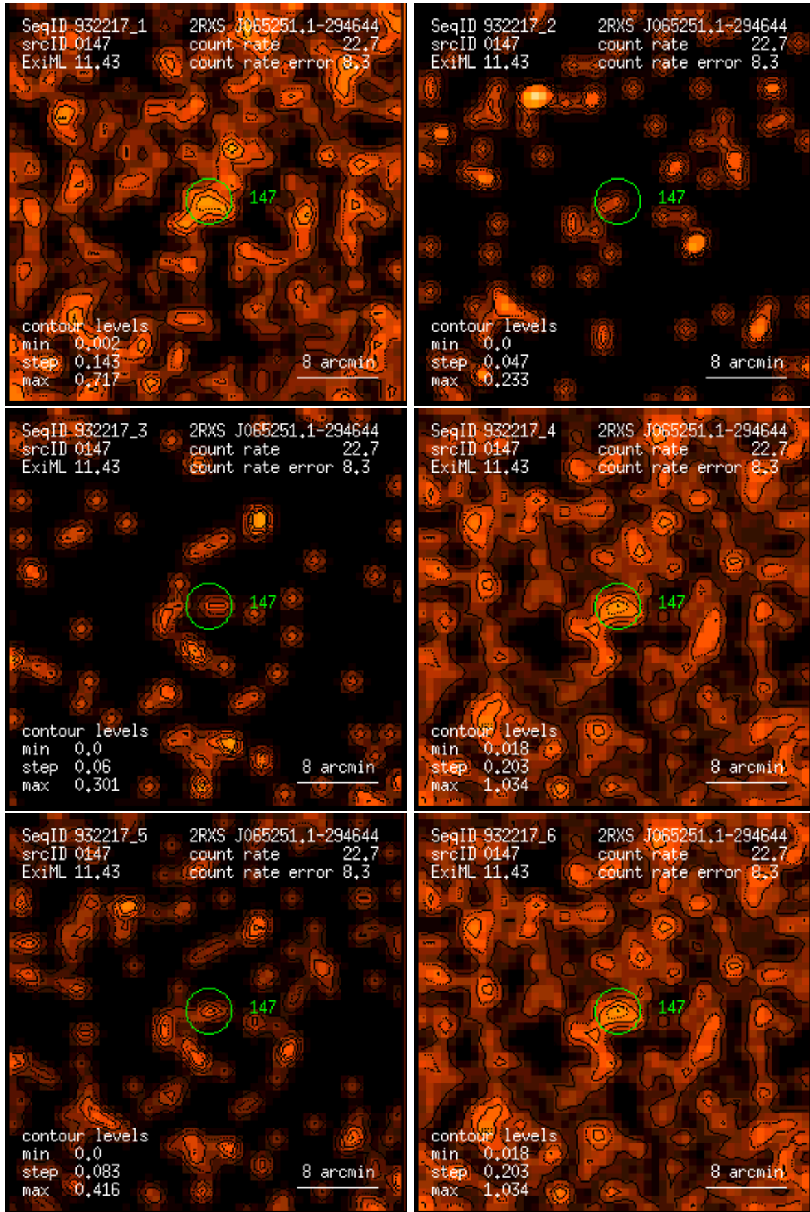
Figure 147: RASS 932217: detection 0147: band rate images, Gaussian filter: (1) PSPC channels 11 – 41, (2) 52 – 90, (3) 91 – 201, (4) 11 – 235, (5) 52 – 201, (6) 11 – 201. Broad band rates in counts/ks. Band rate contour levels in counts/ks/arcmin 2 .
