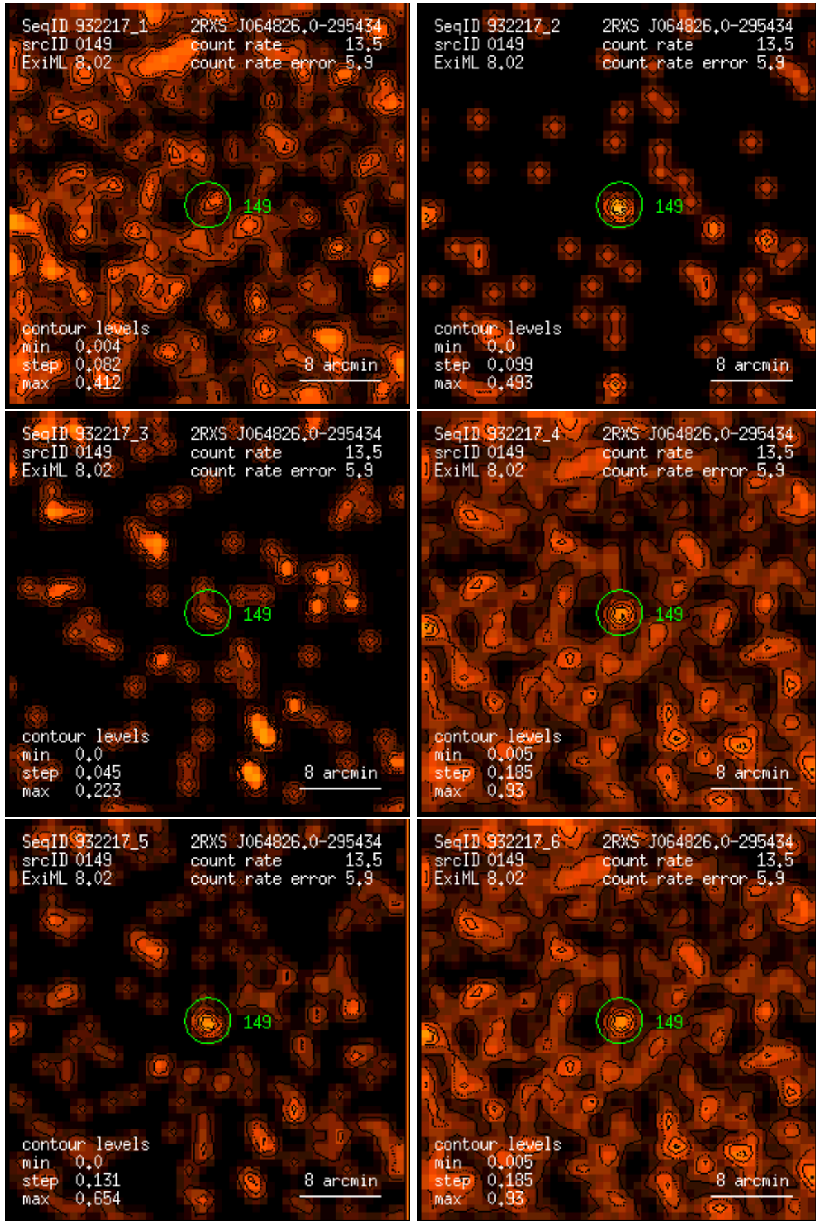
Figure 149: RASS 932217: detection 0149: band rate images, Gaussian filter: (1) PSPC channels 11 – 41, (2) 52 – 90, (3) 91 – 201, (4) 11 – 235, (5) 52 – 201, (6) 11 – 201. Broad band rates in counts/ks. Band rate contour levels in counts/ks/arcmin 2 .
