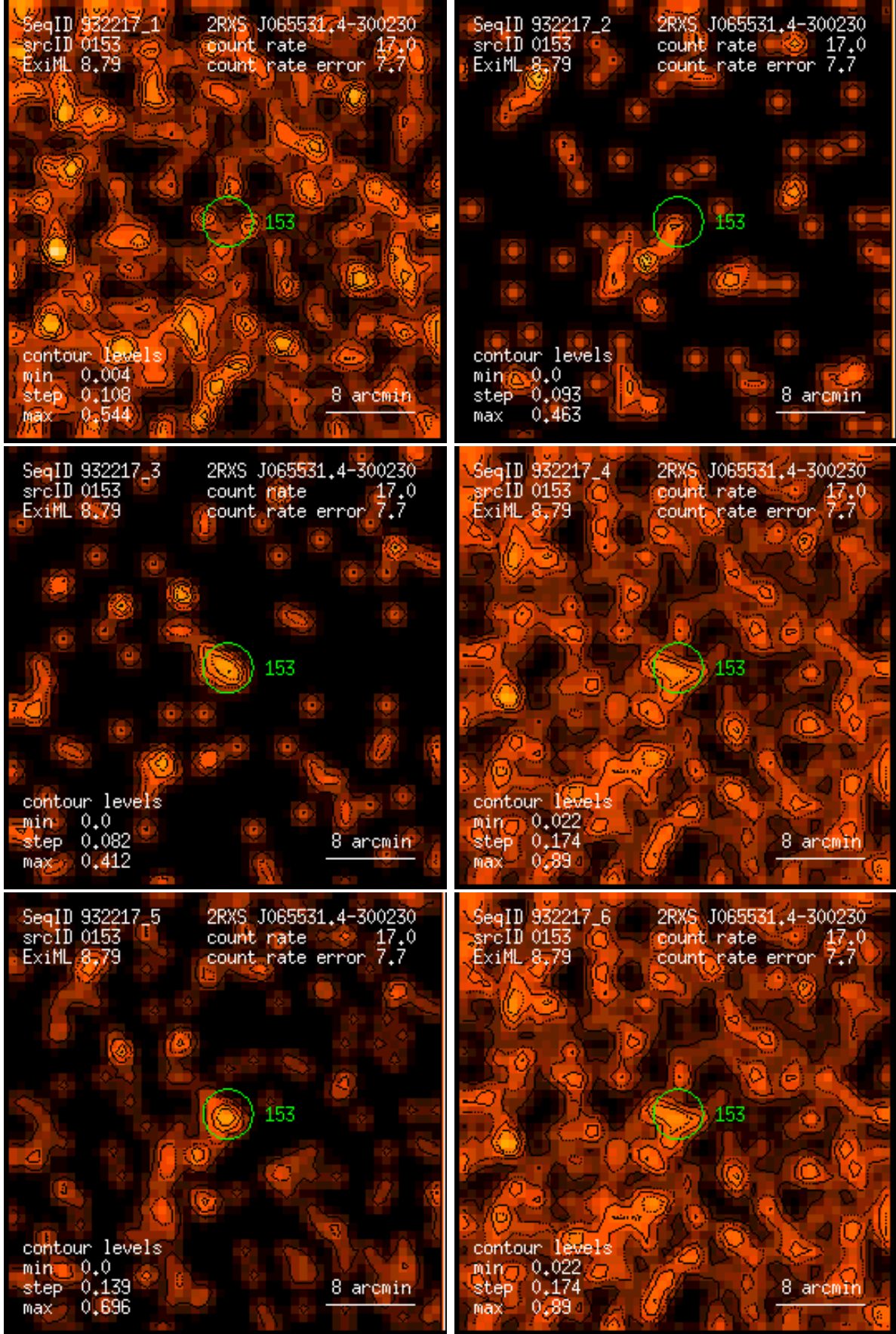
Figure 153: RASS 932217: detection 0153: band rate images, Gaussian filter: (1) PSPC channels 11 – 41, (2) 52 – 90, (3) 91 – 201, (4) 11 – 235, (5) 52 – 201, (6) 11 – 201. Broad band rates in counts/ks. Band rate contour levels in counts/ks/arcmin 2 .
