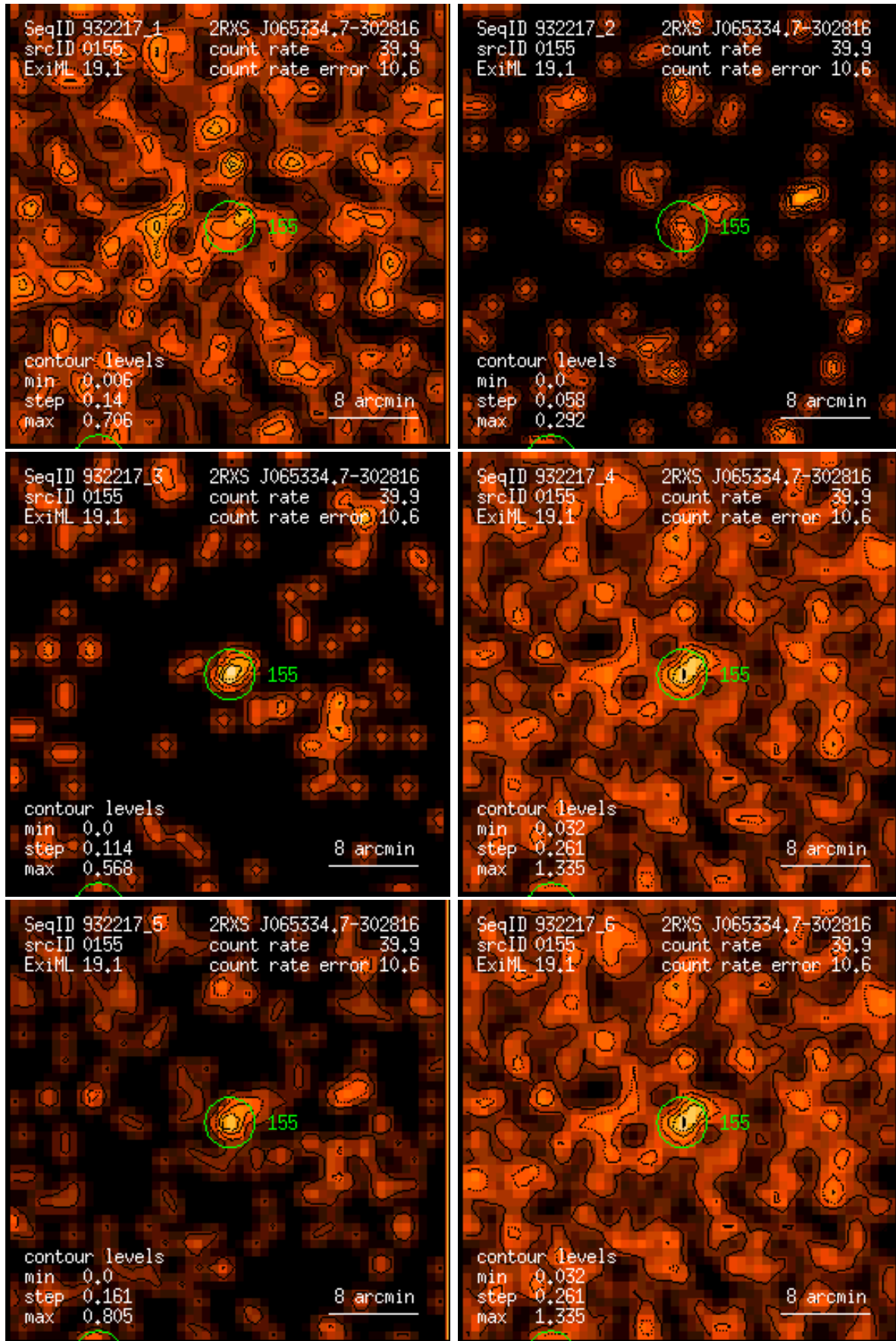
Figure 155: RASS 932217: detection 0155: band rate images, Gaussian filter: (1) PSPC channels 11 – 41, (2) 52 – 90, (3) 91 – 201, (4) 11 – 235, (5) 52 – 201, (6) 11 – 201. Broad band rates in counts/ks. Band rate contour levels in counts/ks/arcmin 2 .
