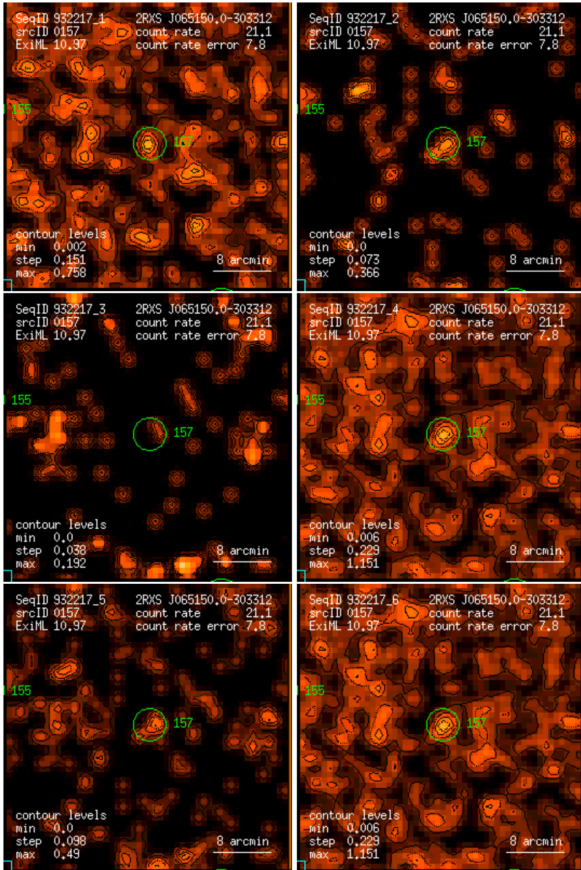
Figure 157: RASS 932217: detection 0157: band rate images, Gaussian filter: (1) PSPC channels 11 – 41, (2) 52 – 90, (3) 91 – 201, (4) 11 – 235, (5) 52 – 201, (6) 11 – 201. Broad band rates in counts/ks. Band rate contour levels in counts/ks/arcmin 2 .
