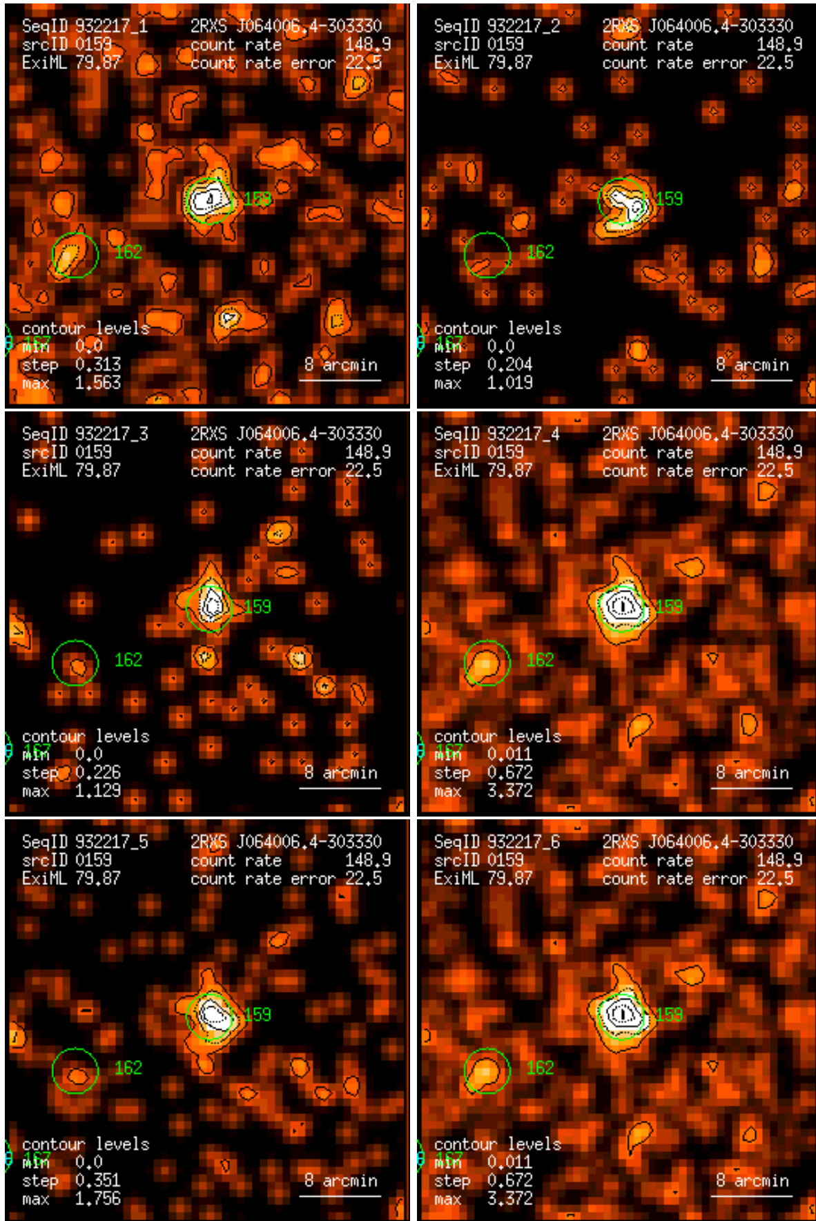
Figure 159: RASS 932217: detection 0159: band rate images, Gaussian filter: (1) PSPC channels 11 – 41, (2) 52 – 90, (3) 91 – 201, (4) 11 – 235, (5) 52 – 201, (6) 11 – 201. Broad band rates in counts/ks. Band rate contour levels in counts/ks/arcmin 2 .
