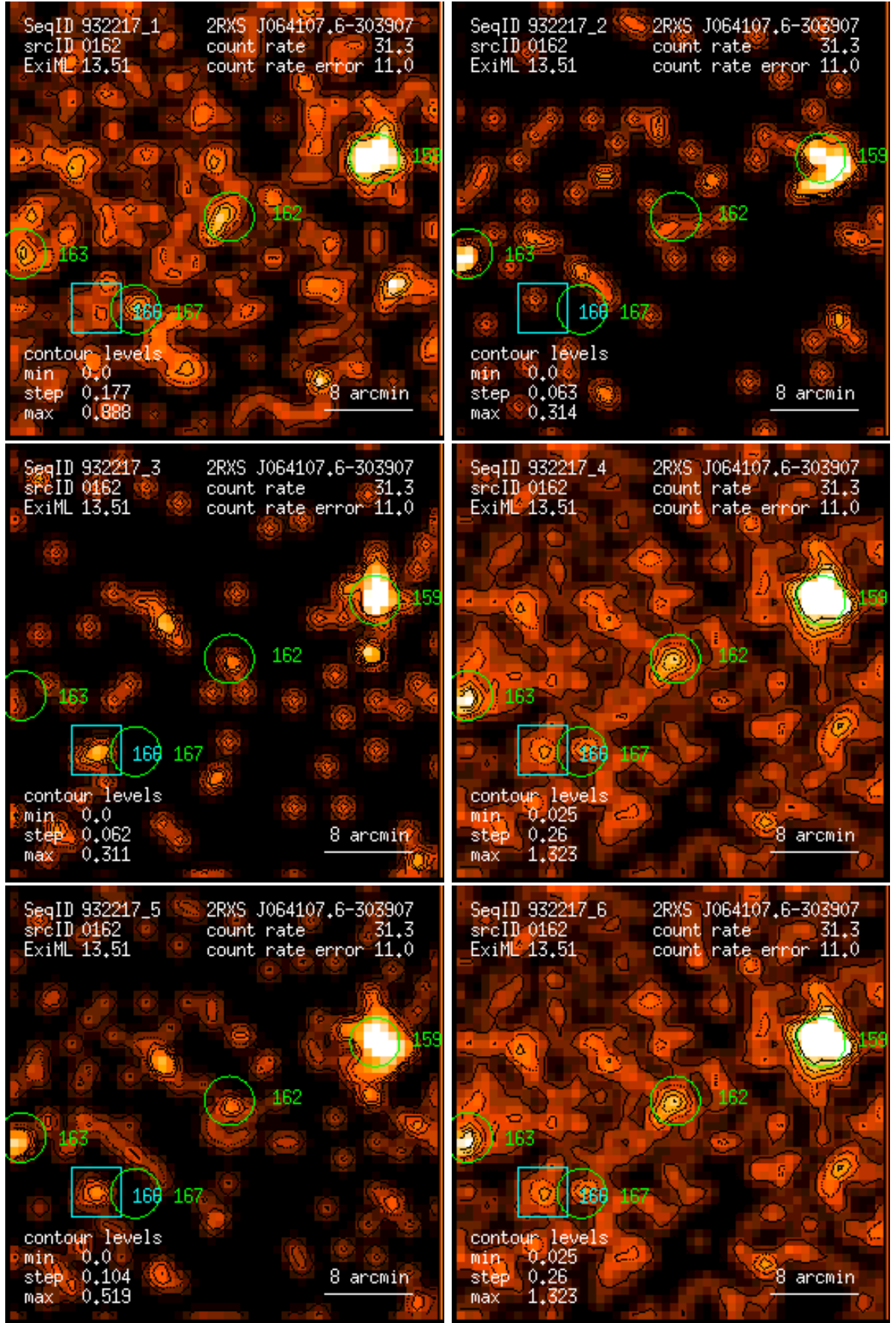
Figure 162: RASS 932217: detection 0162: band rate images, Gaussian filter: (1) PSPC channels 11 – 41, (2) 52 – 90, (3) 91 – 201, (4) 11 – 235, (5) 52 – 201, (6) 11 – 201. Broad band rates in counts/ks. Band rate contour levels in counts/ks/arcmin 2 .
