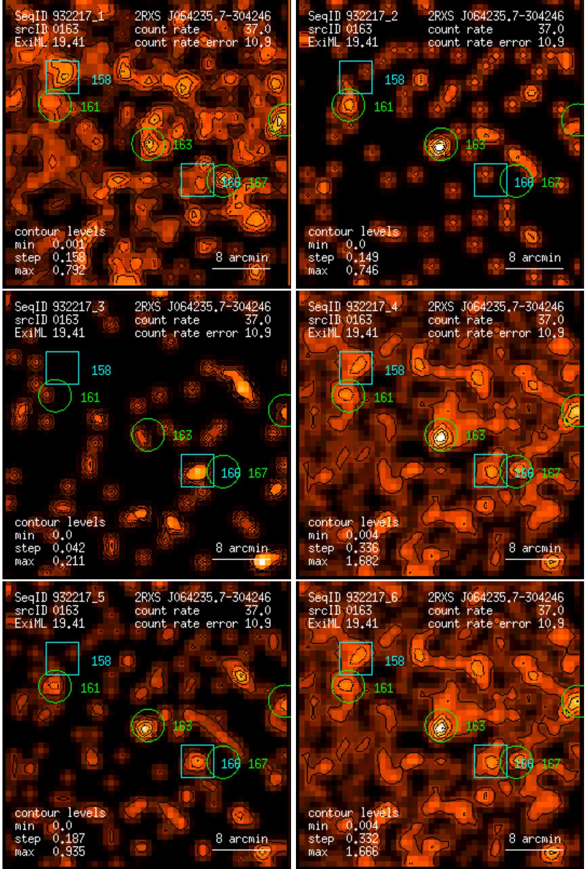
Figure 163: RASS 932217: detection 0163: band rate images, Gaussian filter: (1) PSPC channels 11 – 41, (2) 52 – 90, (3) 91 – 201, (4) 11 – 235, (5) 52 – 201, (6) 11 – 201. Broad band rates in counts/ks. Band rate contour levels in counts/ks/arcmin 2 .
