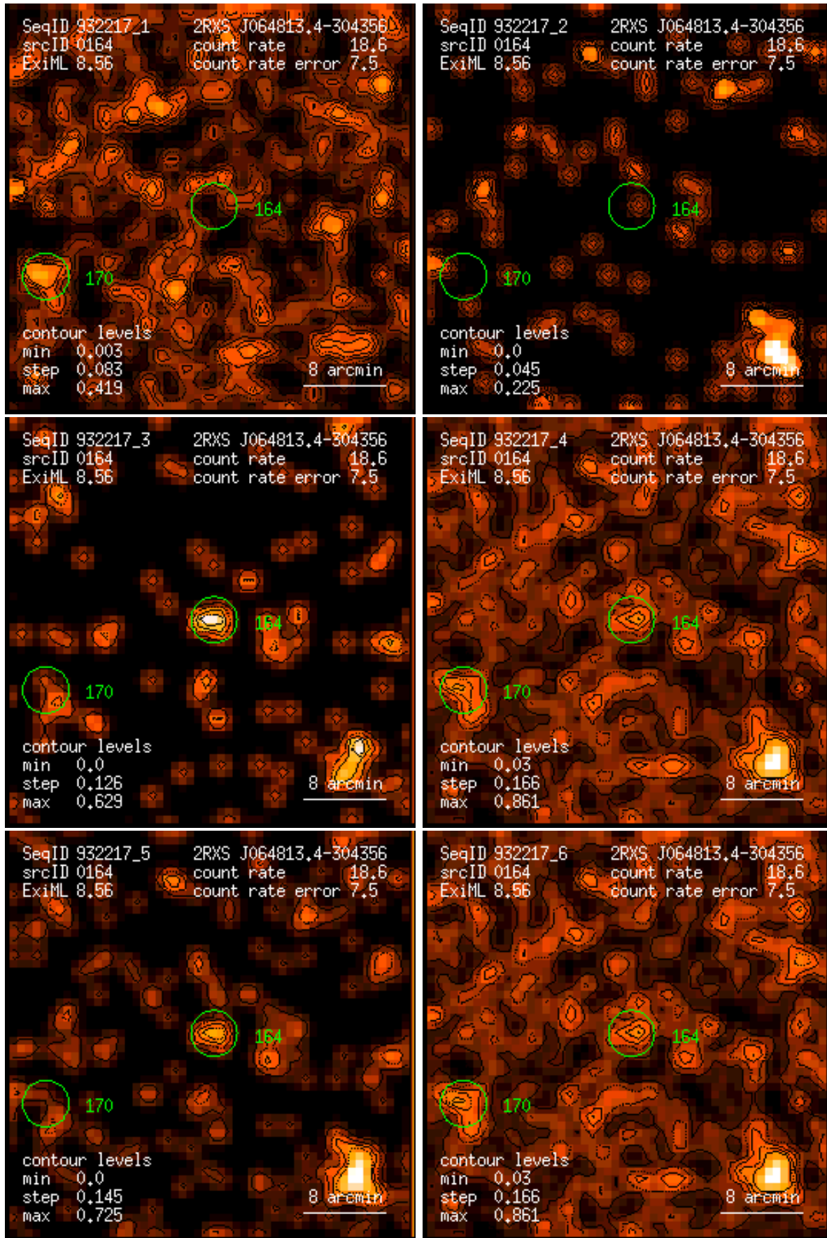
Figure 164: RASS 932217: detection 0164: band rate images, Gaussian filter: (1) PSPC channels 11 – 41, (2) 52 – 90, (3) 91 – 201, (4) 11 – 235, (5) 52 – 201, (6) 11 – 201. Broad band rates in counts/ks. Band rate contour levels in counts/ks/arcmin 2 .
