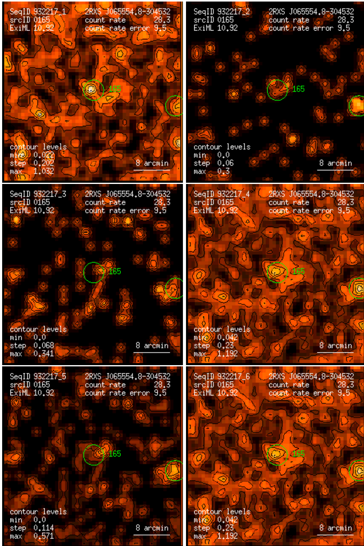
Figure 165: RASS 932217: detection 0165: band rate images, Gaussian filter: (1) PSPC channels 11 – 41, (2) 52 – 90, (3) 91 – 201, (4) 11 – 235, (5) 52 – 201, (6) 11 – 201. Broad band rates in counts/ks. Band rate contour levels in counts/ks/arcmin 2 .
