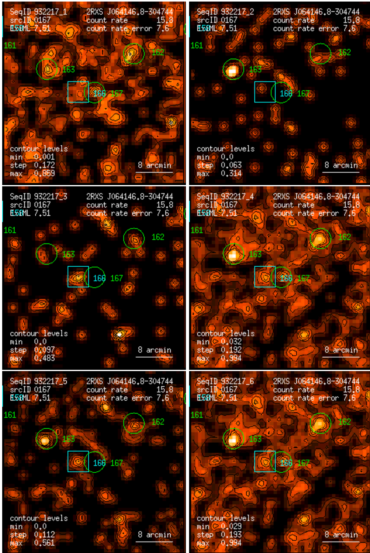
Figure 167: RASS 932217: detection 0167: band rate images, Gaussian filter: (1) PSPC channels 11 – 41, (2) 52 – 90, (3) 91 – 201, (4) 11 – 235, (5) 52 – 201, (6) 11 – 201. Broad band rates in counts/ks. Band rate contour levels in counts/ks/arcmin 2 .
