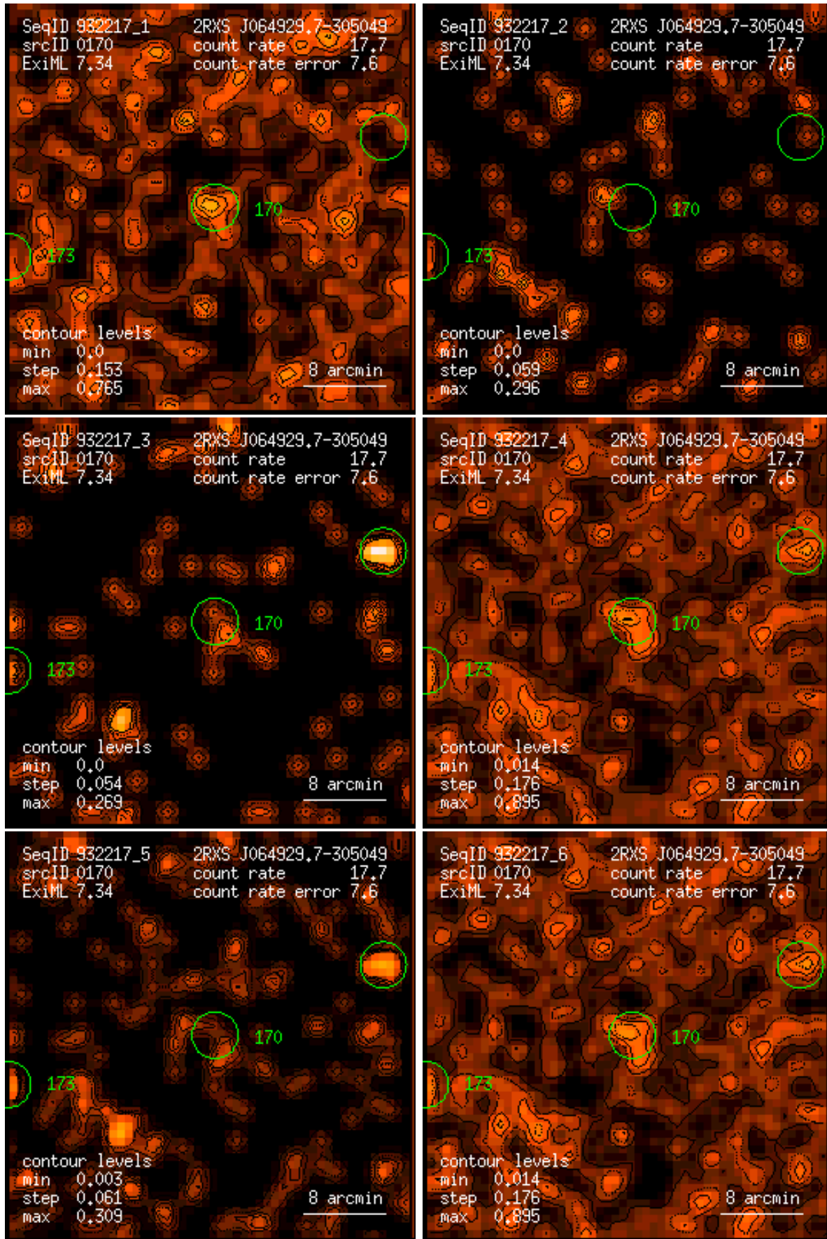
Figure 170: RASS 932217: detection 0170: band rate images, Gaussian filter: (1) PSPC channels 11 – 41, (2) 52 – 90, (3) 91 – 201, (4) 11 – 235, (5) 52 – 201, (6) 11 – 201. Broad band rates in counts/ks. Band rate contour levels in counts/ks/arcmin 2 .
