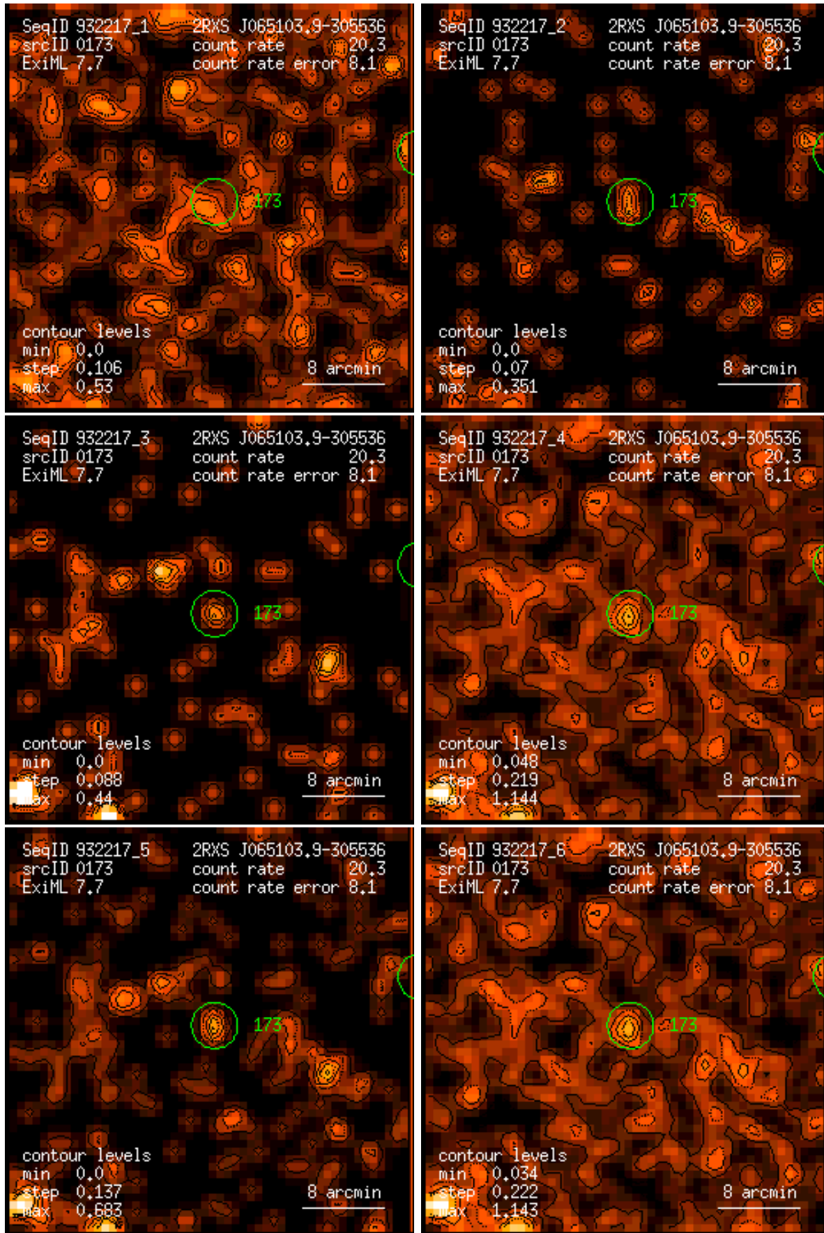
Figure 173: RASS 932217: detection 0173: band rate images, Gaussian filter: (1) PSPC channels 11 – 41, (2) 52 – 90, (3) 91 – 201, (4) 11 – 235, (5) 52 – 201, (6) 11 – 201. Broad band rates in counts/ks. Band rate contour levels in counts/ks/arcmin 2 .
