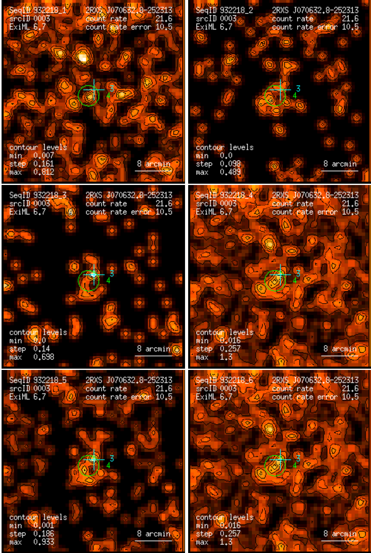
Figure 3: RASS 932218: detection 0003: band rate images, Gaussian filter: (1) PSPC channels 11 – 41, (2) 52 – 90, (3) 91 – 201, (4) 11 – 235, (5) 52 – 201, (6) 11 – 201. Broad band rates in counts/ks. Band rate contour levels in counts/ks/arcmin 2 .
