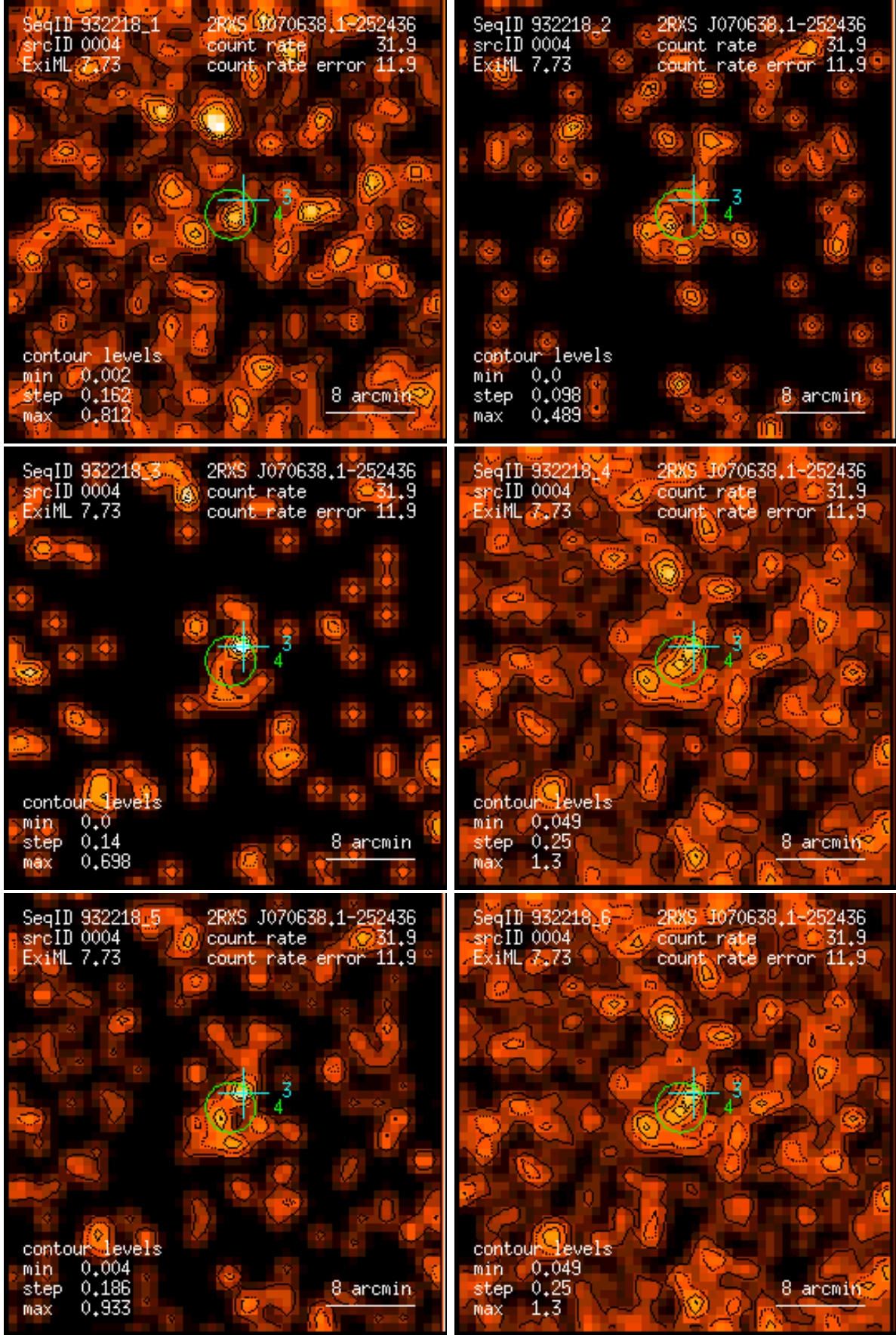
Figure 4: RASS 932218: detection 0004: band rate images, Gaussian filter: (1) PSPC channels 11 – 41, (2) 52 – 90, (3) 91 – 201, (4) 11 – 235, (5) 52 – 201, (6) 11 – 201. Broad band rates in counts/ks. Band rate contour levels in counts/ks/arcmin 2 .
