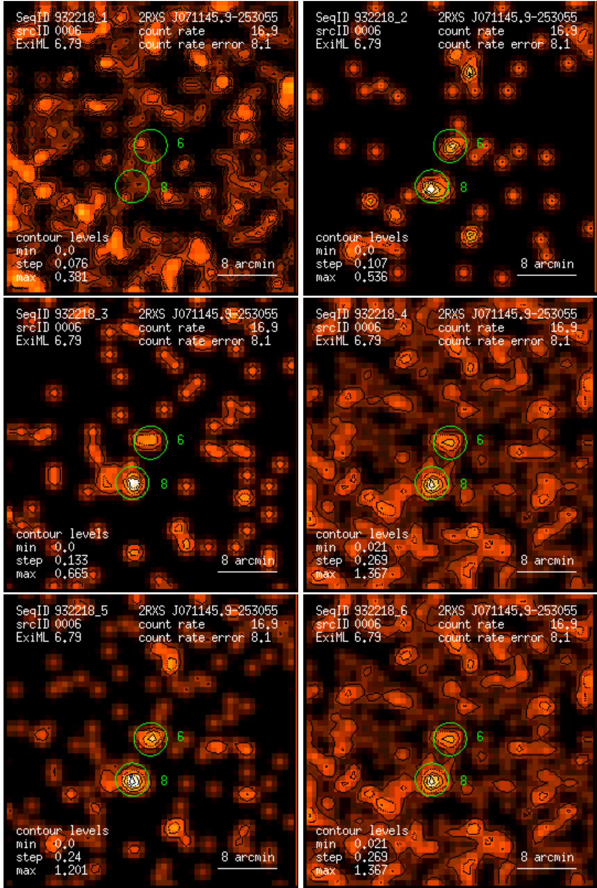
Figure 6: RASS 932218: detection 0006: band rate images, Gaussian filter: (1) PSPC channels 11 – 41, (2) 52 – 90, (3) 91 – 201, (4) 11 – 235, (5) 52 – 201, (6) 11 – 201. Broad band rates in counts/ks. Band rate contour levels in counts/ks/arcmin 2 .
