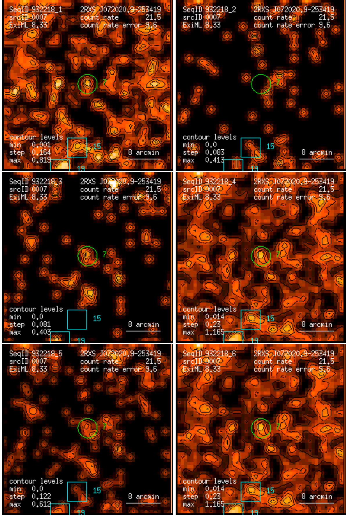
Figure 7: RASS 932218: detection 0007: band rate images, Gaussian filter: (1) PSPC channels 11 – 41, (2) 52 – 90, (3) 91 – 201, (4) 11 – 235, (5) 52 – 201, (6) 11 – 201. Broad band rates in counts/ks. Band rate contour levels in counts/ks/arcmin 2 .
