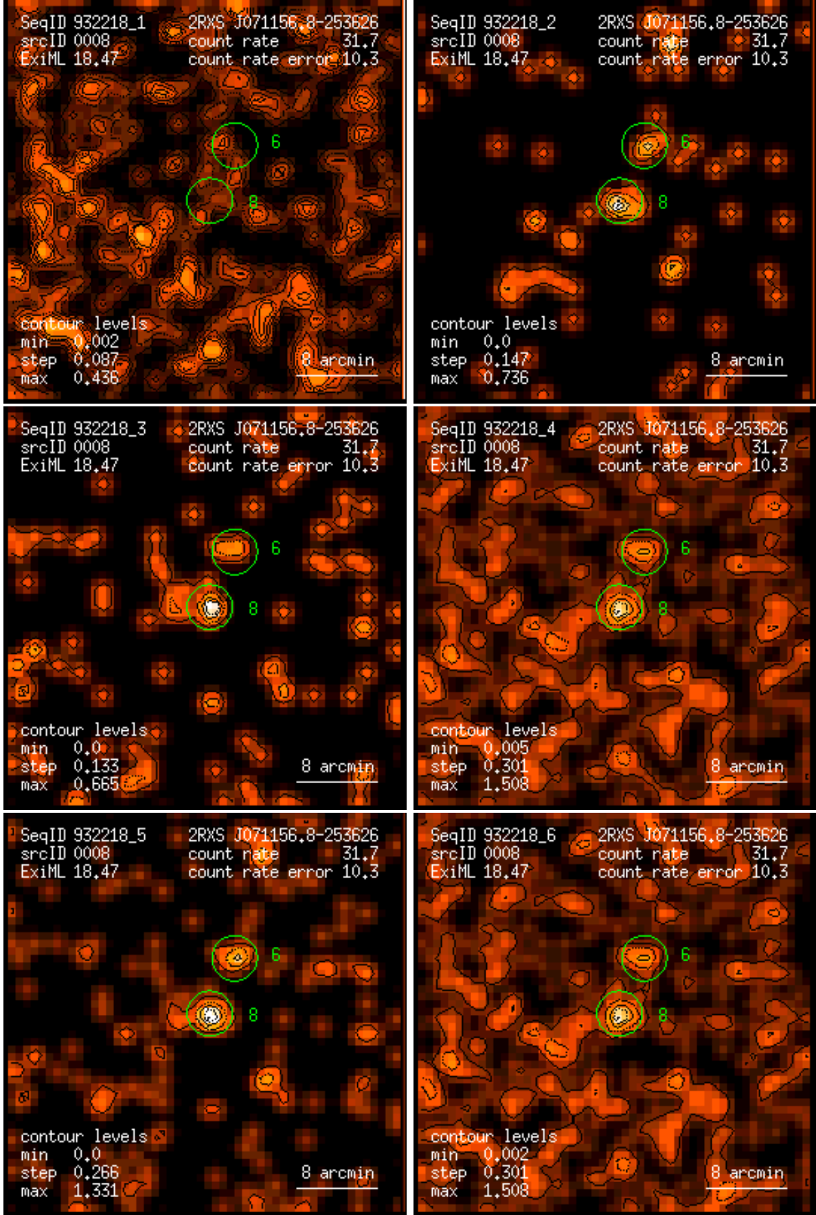
Figure 8: RASS 932218: detection 0008: band rate images, Gaussian filter: (1) PSPC channels 11 – 41, (2) 52 – 90, (3) 91 – 201, (4) 11 – 235, (5) 52 – 201, (6) 11 – 201. Broad band rates in counts/ks. Band rate contour levels in counts/ks/arcmin 2 .
