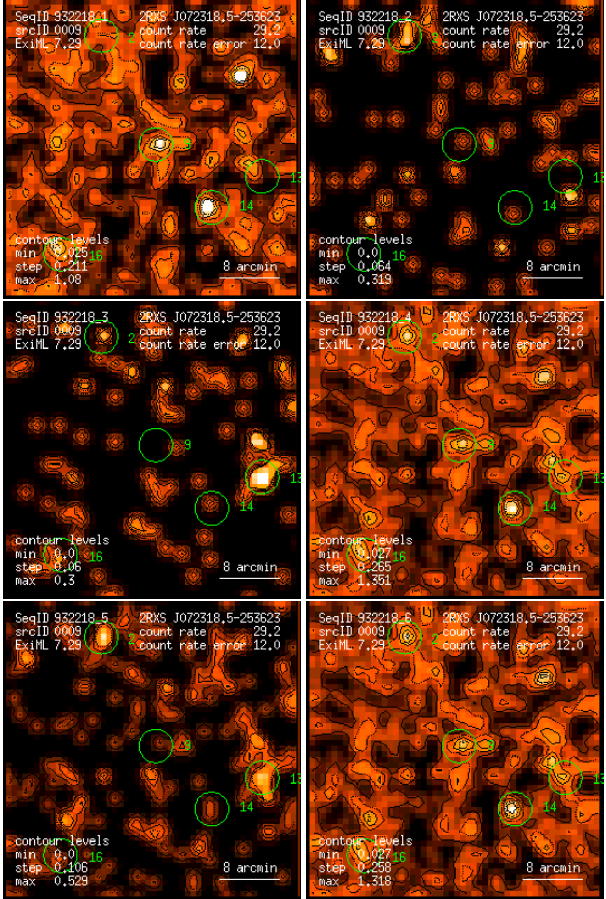
Figure 9: RASS 932218: detection 0009: band rate images, Gaussian filter: (1) PSPC channels 11 – 41, (2) 52 – 90, (3) 91 – 201, (4) 11 – 235, (5) 52 – 201, (6) 11 – 201. Broad band rates in counts/ks. Band rate contour levels in counts/ks/arcmin 2 .
